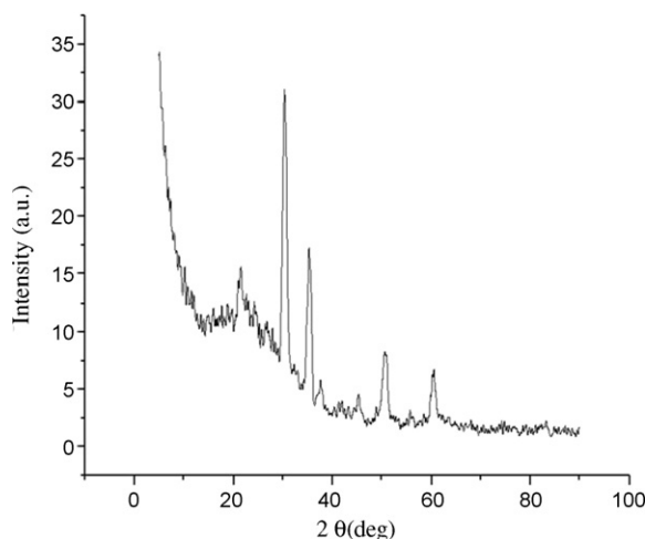
Fig. 3. X-ray diffraction image of nano-TiO 2 particles.
