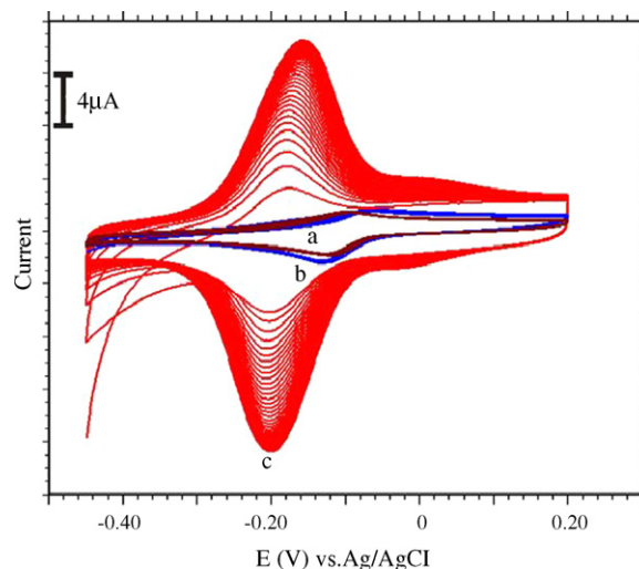
Fig. 7. CVs of TN deposition onto DNA/nano- \text{TiO}_2 /GCE (c), bare GCE (b) and nano- \text{TiO}_2 /GCE (a) from PBS (pH 7.0) containing 1 \times 10^{-5} M TN.
