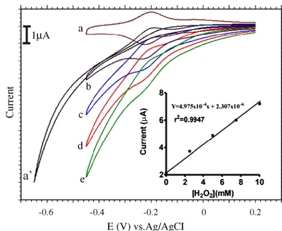
Fig. 6. Electrocatalytic reduction of \text{H}_2\text{O}_2 in pH 7.0 PBS at TN/DNA/nano- \text{TiO}_2 /GCE. (a) 0.0 M, (b) 2.5 \times 10^{-3} M, (c) 5 \times 10^{-3} M, (d) 7.5 \times 10^{-3} M, (e) 1 \times 10^{-2} M \text{H}_2\text{O}_2 and (a') nano- \text{TiO}_2 /GCE in 1 \times 10^{-2} M \text{H}_2\text{O}_2 .
