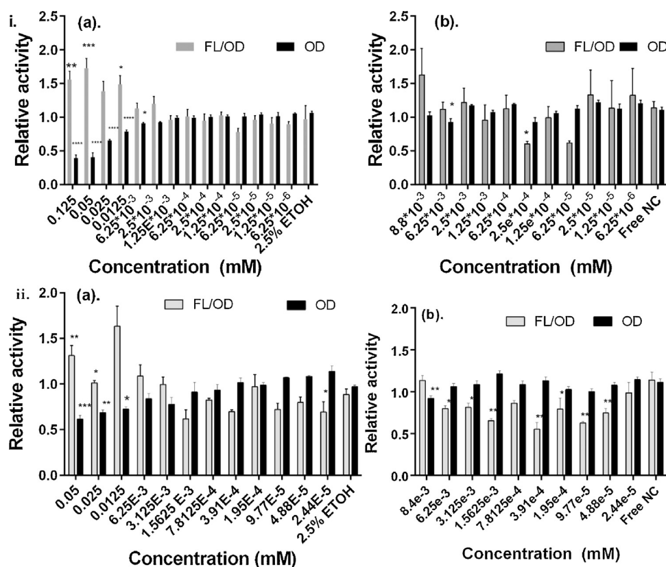
Fig. 2. Effect of varying doses of baicalein (i) and quercetin (ii) as (a) free solution, and (b) loaded nanocapsules on the relative growth ( OD_{600} ) and relative quorum sensing activity ( FL/OD_{600} ), evaluated in a E. coli Top 10 quorum sensing biosensor strain. Average values represent average \pm S.D. (n=3).
