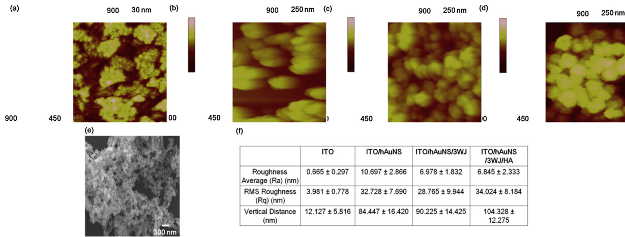
Fig. 3. (a) Surface morphology of ITO substrate by AFM (b) hAuSN-immobilized on ITO substrate by AFM, (c) surface morphology of DNA 3 W J on hAuSN-immobilized ITO substrate by AFM, (d) Surface morphology of HA protein on DNA 3 W J /hAuSN/ITO by AFM, (e) Surface morphology of hAuSN-immobilized substrate by FE-SEM, (f) Surface roughness analysis of the ITO, hAuSN/ITO, DNA 3 W J /hAuSN/ITO and HA protein/ DNA 3 W J /hAuSN/ITO.
