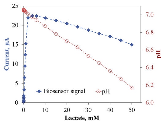
Fig. 4. LO x -Cu-MOF/CS/Pt/SPCE biosensor kinetic registered at + 0.15 V (vs SPE Ag/AgCl) and pH variation with lactate concentration in supporting electrolyte (0.1 M PB at pH 7.0).
