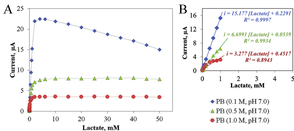
Fig. 5. Influence of phosphate buffer concentration in the amperometric signal. (A) Current registered at + 0.15 V (vs Ag/AgCl), using the LO x -Cu-MOF/CS/Pt/SPCE biosensor; (B) Variation of the calibration curves' slope with the phosphate concentration in supporting electrolyte.
