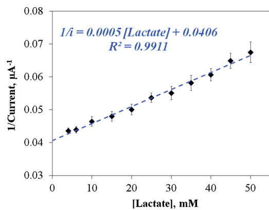
Fig. 3. Determination of the crosslinked LO x kinetic parameters in inhibition range assuming a rapid equilibrium. Representation of 1/i vs [S] , in lactate additions at PB (0.1 M, pH 7.0) (n = 5).
