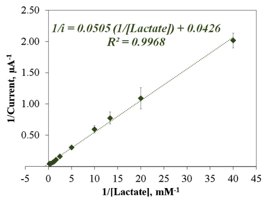
Fig. 2. Determination of the crosslinked LO x kinetic constants. Lineweaver-Burk model fitting to the catalytic range using the amperometric response for lactate additions at 0.1 M PB, pH 7.0 (n = 5).
