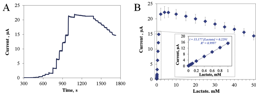
Fig. 1. Electrochemical response of \text{LO}_x\text{-Cu-MOF/CS/Pt/SPCE} biosensor. (A) Amperogram registered at + 0.15 V (vs SPE Ag/AgCl) for successive additions of lactate in PB (0.1 M, pH 7.0); and (B) Plotting of current vs lactate concentration ( n = 5 ). Inset: calibration curve for lactate concentration range from 0 to 1.0 mM.
