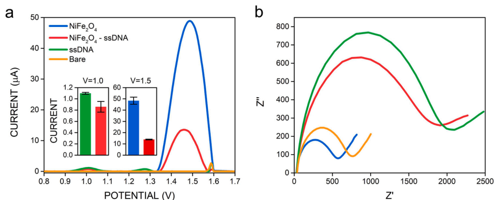
Fig. 5. (a) Differential Pulse Voltammogram, (inset) histogram for the oxidation peak currents of guanine bases of ssDNA (at +1.0 V) and the NiFe 2 O 4 nanoparticles (at +1.5 V) before and after interaction with each other. (b) Electrochemical Impedance Spectra for bare, ssDNA coated, and NiFe 2 O 4 nanoparticle-modified electrodes before and after interaction with each other.
