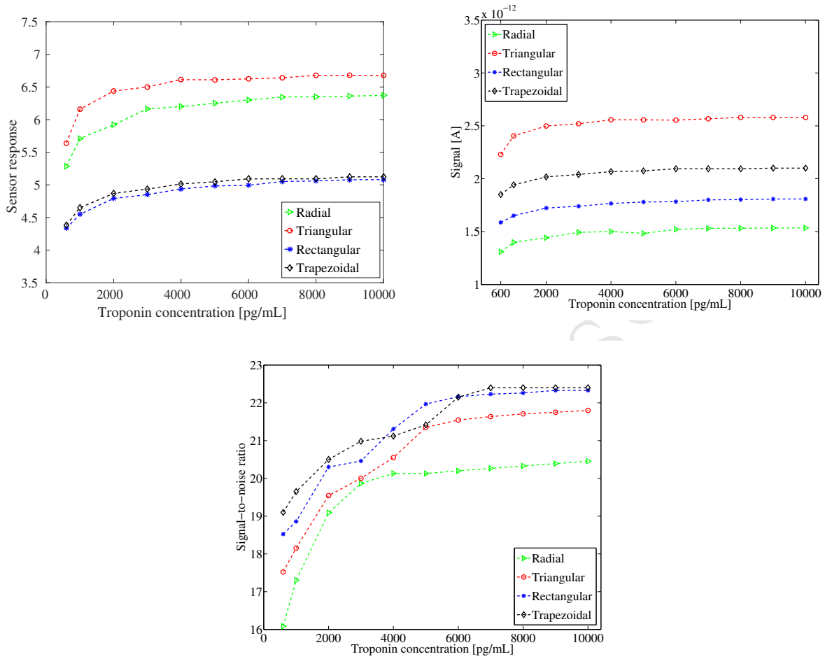
Figure 10: Sensitivity (top left), signal (top right), and SNR (bottom) as a function of troponin concentration varying from 500 pg/mL and 10 ng/mL for different nanowires cross sections. The sensor is 1000 nm wide and the bulk oxide is 300 nm thick. Each sensor has four parallel 5000 nm long nanowires, a cross-sectional area of 2500 nm 2 , a doping concentration of 10^{17} cm -3 , and they are protected by a 5 nm thick silicon oxide layer.
