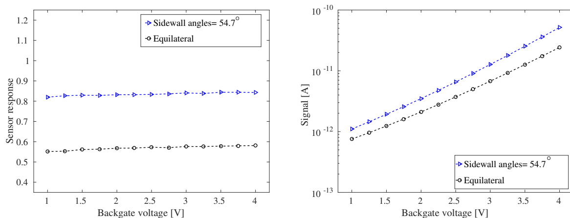
Figure 6: Sensor response (left) and signal (right) of two triangular nanowires for different backgate voltages at 10 pg/mL troponin concentration. The sensors are 300 nm wide and the bulk oxide is 200 nm thick. Each sensor has one 1000 nm long nanowire, a cross-sectional area of 2500 nm 2 , a doping concentration of 10 17 cm -3 , and they are protected by a 5 nm thick silicon oxide layer.
