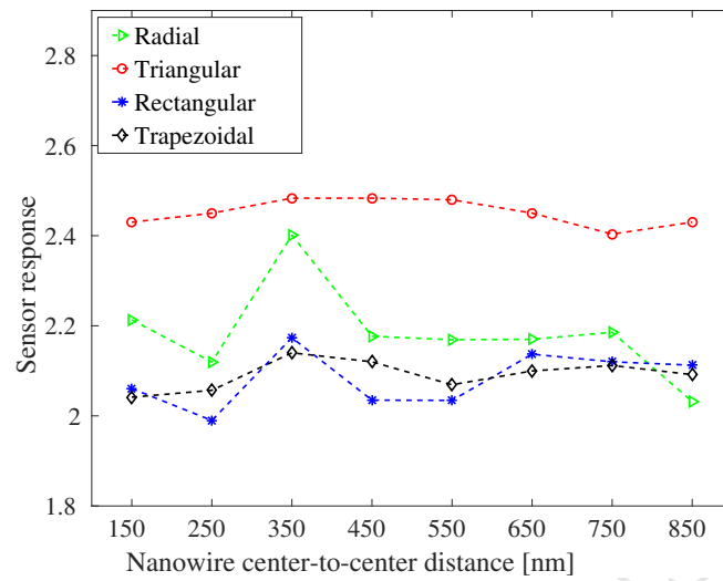
Figure 9: The sensor response of different devices as a function of the nanowire center-to-center distance at 75 pg/ml cTn concentration. The sensors are 1000 nm wide and the bulk oxide is 300 nm thick. Each sensor has two parallel 5000 nm long nanowires, a cross-sectional area of 2500 nm 2 , a doping concentration of 10 17 cm -3 , and they are protected by a 5 nm thick silicon oxide layer.
