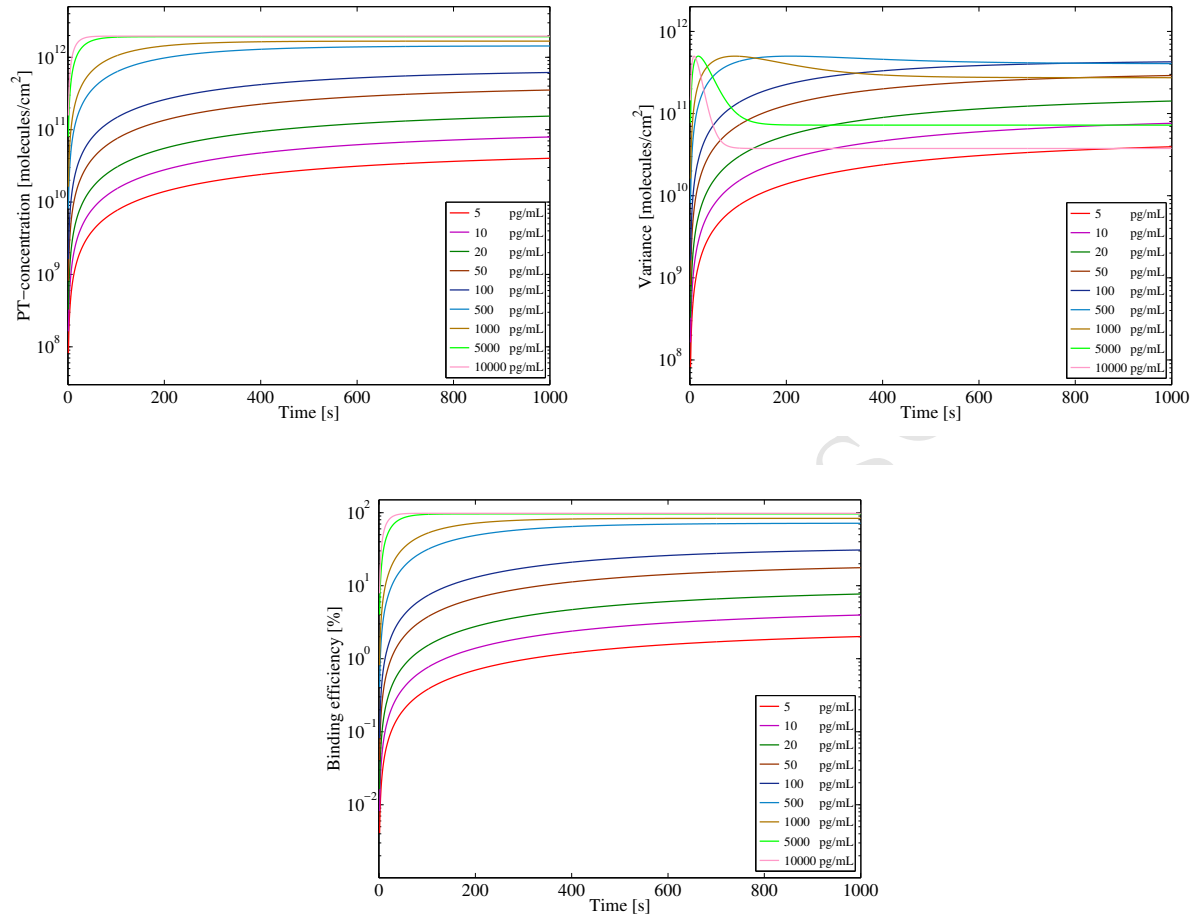
Figure 3: The expected value (top left), variance (top right), and binding efficiency (bottom) of PT -complexes for different troponin concentrations.
