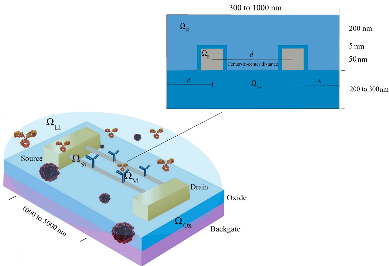
Figure 1: Schematic diagram of the nanowire field-effect sensor showing receptor and target molecules. The subdomains, i.e., silicon nanowire \Omega_{Si} , insulator \Omega_{Ox} , the specific binding of target to probe molecules \Omega_M , and the electrolyte \Omega_{El} are illustrated with their dimensions and ranges. Additionally, d indicates the center-to-center distance between the nanowires and d_1 is the distance between a nanowire and the boundary.
