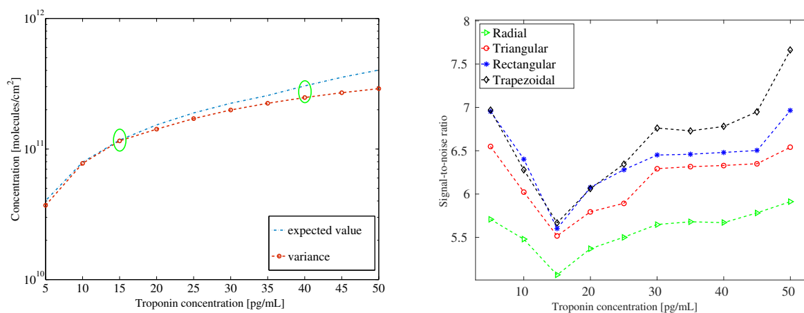
Figure 5: Expected value and variance of PT -complexes (left) and signal-to-noise ratio (right) as a function of troponin concentration varying from 5 pg/ml and 50 pg/ml for different nanowire cross sections. The sensors are 300 nm wide and the bulk oxide is 200 nm thick. Each sensor has one 1000 nm long nanowire, a cross-sectional area of 2500 nm 2 , a doping concentration of 10 17 cm -3 , and they are protected by a 5 nm thick silicon oxide layer.
