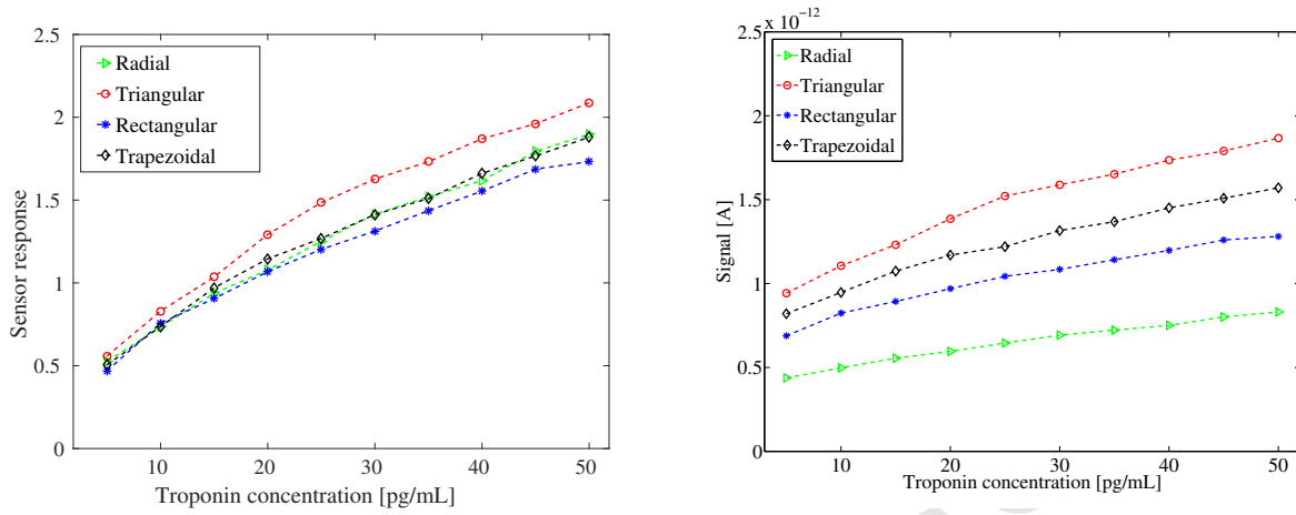
Figure 4: Sensor response (left) and signal (right) as a function of troponin concentration varying from 5 pg/ml and 50 pg/ml for different nanowire cross sections. The sensors are 300 nm wide and the bulk oxide is 200 nm thick. Each sensor has one 1000 nm long nanowire, a cross-sectional area of 2500 nm 2 , a doping concentration of 10 17 cm -3 , and they are protected by a 5 nm thick silicon oxide layer.
