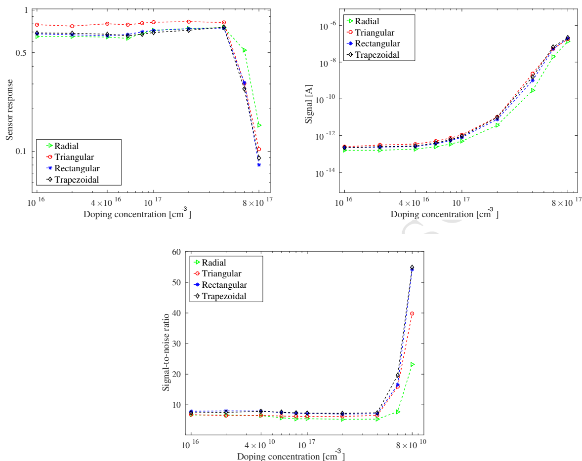
Figure 7: Sensor response (top left), signal (top right), and SNR (bottom) as a function of doping concentration for different nanowire cross sections. The sensors are 300 nm wide and the bulk oxide is 200 nm thick. Each sensor has one 1000 nm long nanowire, a cross-sectional area of 2500 \text{ nm}^2 and they are protected by a 5 nm thick silicon oxide layer.
