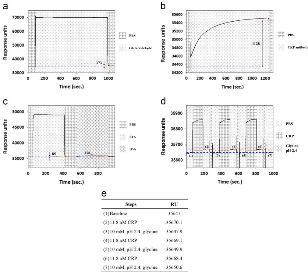
Fig. 4. SPR measurement data for the antiCRP-CRP interaction: (a) during activation, (b) during immobilization, (c) during blocking, (d) during regeneration (Note: red dashed line represents the signal after antigen binding and the blue dotted line represents the signal after regeneration), and (e) RU during regeneration in item (d).
