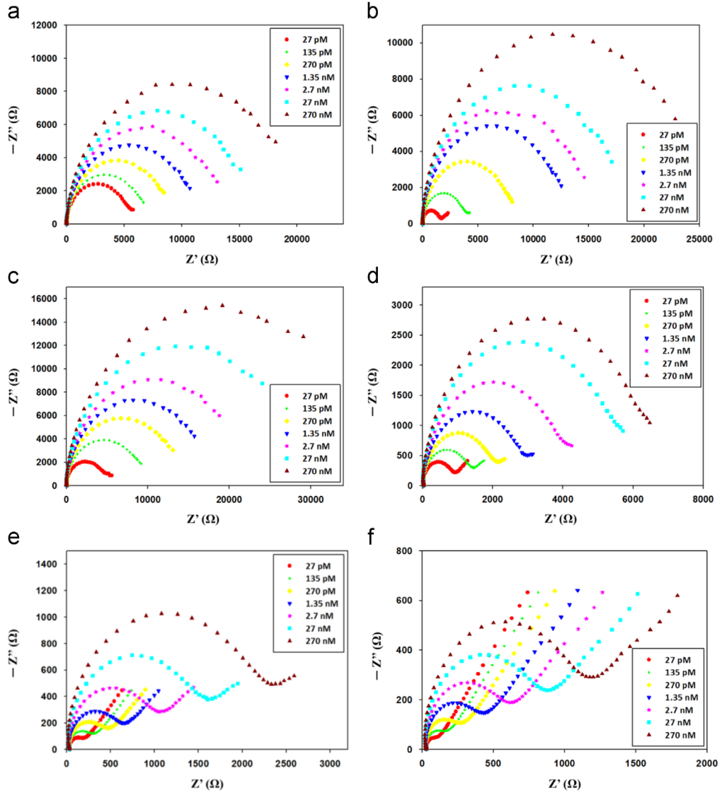
Fig. 1. Impedance data of the linker/glutaraldehyde/antibody/ETA&BSA modified electrode in a 1× PBS solution with 1 mM Fe (CN) 6 3-/4- after addition of the target protein at different concentrations: (a) 4-ATP, antiS100, and S100 beta protein in Nyquist form of interdigitate biochip, (b) 4-ATP, antiS100, and S100 beta protein in Nyquist form of interdigitate-semicircle biochip, (c) 4-ATP, antiS100, and S100 beta protein in Nyquist form of interdigitate-zigzag biochip, (d) 4-ATP, antiCRP, and CRP in Nyquist form of interdigitate-zigzag biochip, (e) cysteamine, antiS100, and S100 beta protein in Nyquist form of interdigitate-zigzag biochip, and (f) cysteamine, antiCRP, and CRP in Nyquist form of interdigitate-zigzag biochip.
