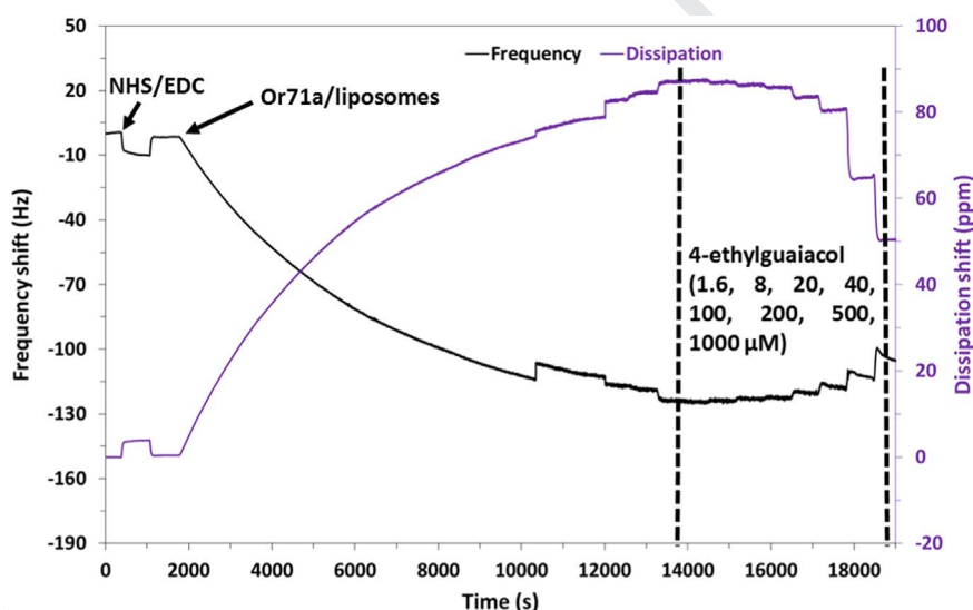
Fig. 2. Change in frequency and dissipation of a gold surface with self-assembled monolayers (SAMs) of 6-mercaptopentanoic acid (MHA) and N-hydroxysuccinimide (NHS)/1-ethyl-3-(3-dimethylaminopropyl)-carbodiimide (EDC) modification, followed by Or71a/liposome immobilization on the QCM sensor and then binding of the target ligand 4-ethylguaiaicol.
