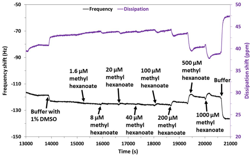
Fig. 5. Close up view of the change in frequency and dissipation with increasing concentrations of methyl hexanoate (0, 1.6, 8, 20, 40, 100, 200, 500 and 1000 \mu\text{M} ) for the Or22a/liposome QCM sensor.
