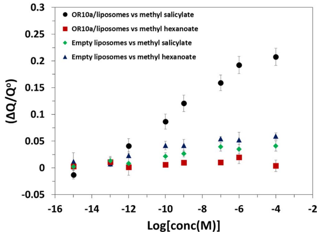
Fig. 8. Dose response curve in terms of change in normalized capacitance values for Or10a/liposomes on an EIS based sensor showing detection of its specific ligand methyl salicylate with high selectivity and sensitivity. Error bars; standard deviation (SD) were generated using four repeats.
