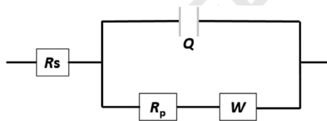
Fig. 6. Equivalent circuit diagram (Randles model) for fitting the non-Faradaic impedance curves where R_s is solution resistance, Q refers to capacitance, R_p is called polarization resistance and W refers to Warburg diffusion.
