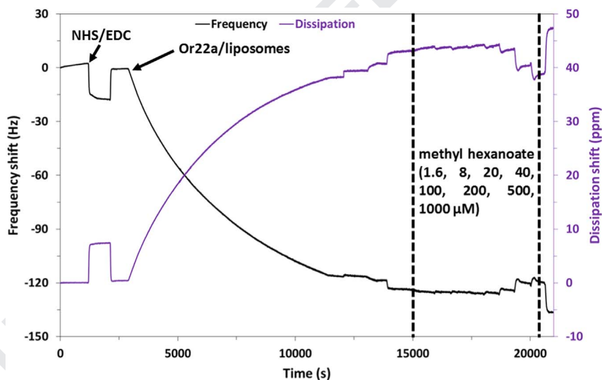
Fig. 4. Change in frequency and dissipation of gold surface with SAM and NHS/EDC modification, followed by Or22a/liposome immobilization on the QCM sensor and then binding of the target ligand methyl hexanoate.
