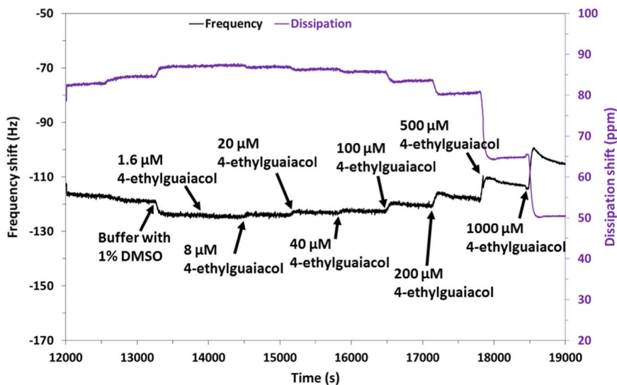
Fig. 3. Close up view of the change in frequency and dissipation with increasing concentrations of 4-ethylguaiaicol (0, 1.6, 8, 20, 40, 100, 200, 500 and 1000 \mu\text{M} ) for the Or71a/liposome QCM sensor.
