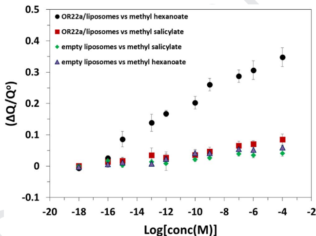
Fig. 9. Dose response curve in terms of change in normalized capacitance values for Or22a/liposomes on an EIS based sensor showing detection of its specific ligand methyl hexanoate with high selectivity and sensitivity. Error bars; standard deviation (SD) were generated using four repeats.
