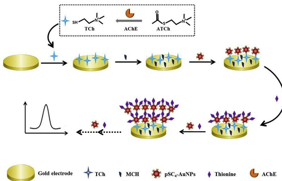
Fig. 7. Schematic of thionine mediated p-SCX4 capped AuNPs multilayers signal amplification on the electrode surface [85]. (Reprint license number: 4710030777146).
