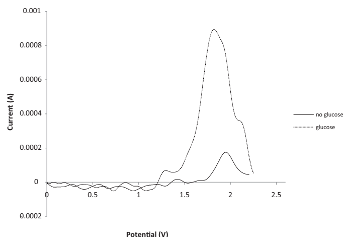
Fig. 12. Electrochemical behavior of chitosan membrane with and without glucose in the test solution. (First configuration electrode, scan rate of 0.01 V/s, potential range from 0 to 2.5 V).
