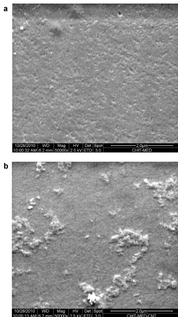
Fig. 4. Visualization of surface morphology using SEM. (a) Chitosan only (b) Chitosan – CNT.
