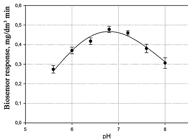
Fig. 5. Dependence of the response of a D. hanseni -based biosensor on pH.
