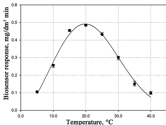
Fig. 7. Dependence of the response of a biosensor based on the yeast D. hanseni on temperature.
