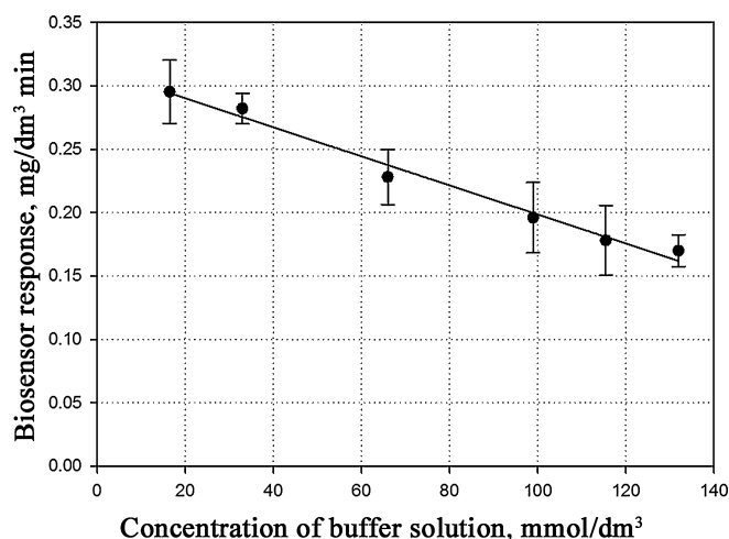
Fig. 6. Dependence of the response of a D. hanseni -based biosensor on the ionic strength of solution.
