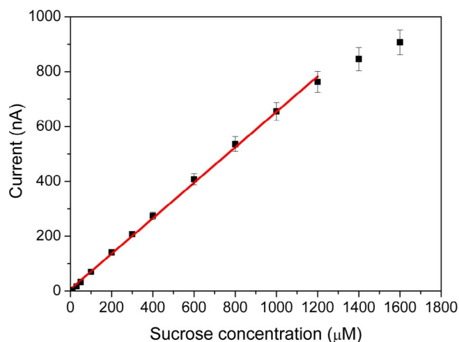
Fig. 2. Calibration curve obtained for the sucrose biosensor. Experimental conditions: 0.5 mM Azure C, 0.1 M phosphate buffer, pH 5.75, applied potential –100 mV vs. Ag/AgCl.
