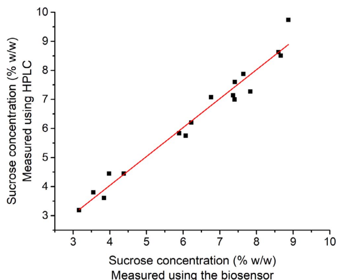
Fig. 3. Graphical comparison between the sucrose determination in 17 green coffee sample, performed using the proposed electrochemical biosensor and the comparative HPLC methodology.
