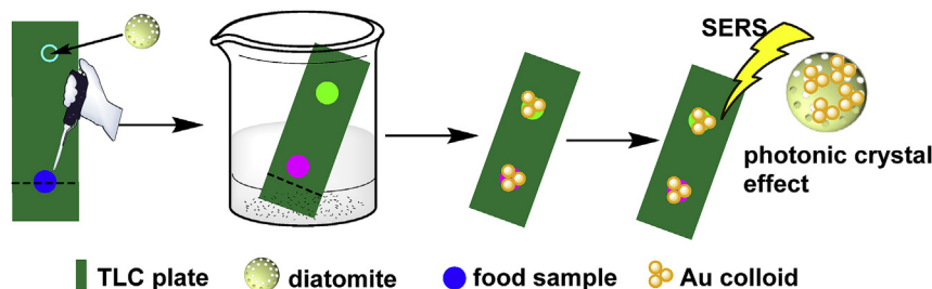
Scheme 1. Schematic representation of the TLC-SERS detection of target molecule from food product base on diatomite TLC plate.
