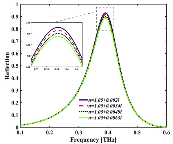
Figure 4. The simulated results of reflectance spectrum for different imaginary parts of the CRI of the surrounding medium.
