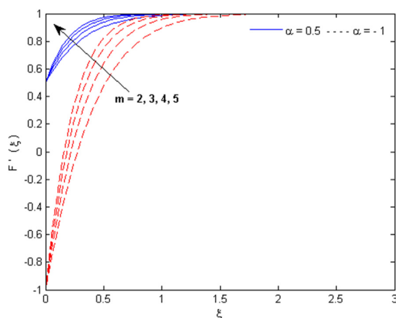
Figure 3. Velocity profile for various m and \alpha .
