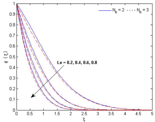
Figure 9. Concentration profile for various Le and N_b .
