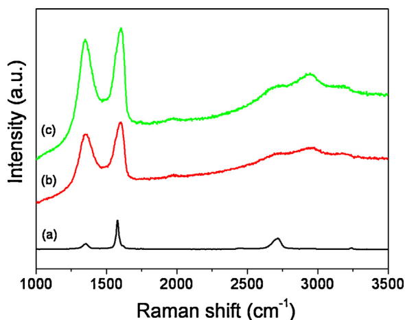
Fig. 2. Raman spectra of graphite (a), pristine graphene oxide (b), and chitosan/graphene oxide bionanocomposite (c).
