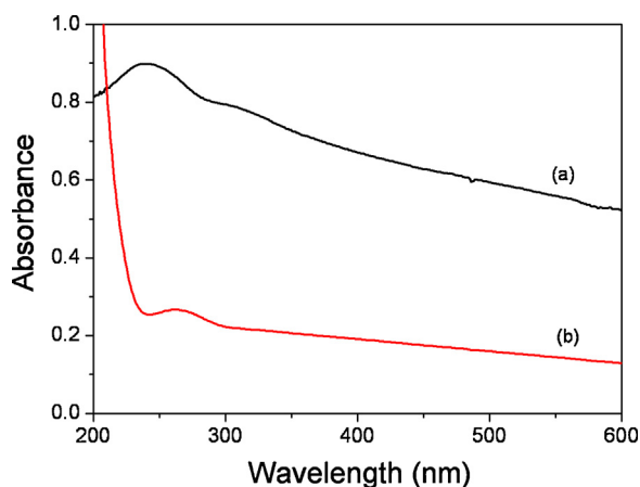
Fig. 6. UV-vis spectra of pristine graphene oxide (a) and chitosan/graphene oxide (b).
