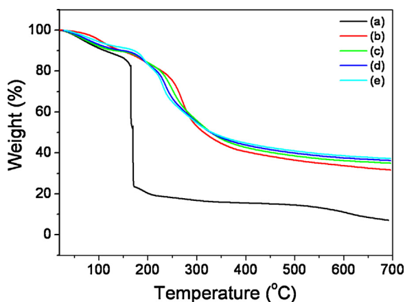
Fig. 3. TGA of pristine graphene oxide (a), pure chitosan film (b) and chitosan/graphene oxide 0.030 (c), 0.060 (d) and 0.120 (e) bionanocomposite.
