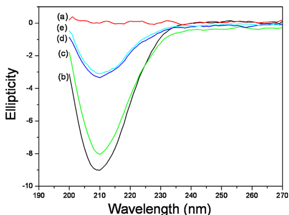
Fig. 7. CD spectra of pristine graphene oxide (a), pure chitosan (b), chitosan/graphene oxide at pH 6.31 (c), 4.29 (d) and 4.20 (e).
