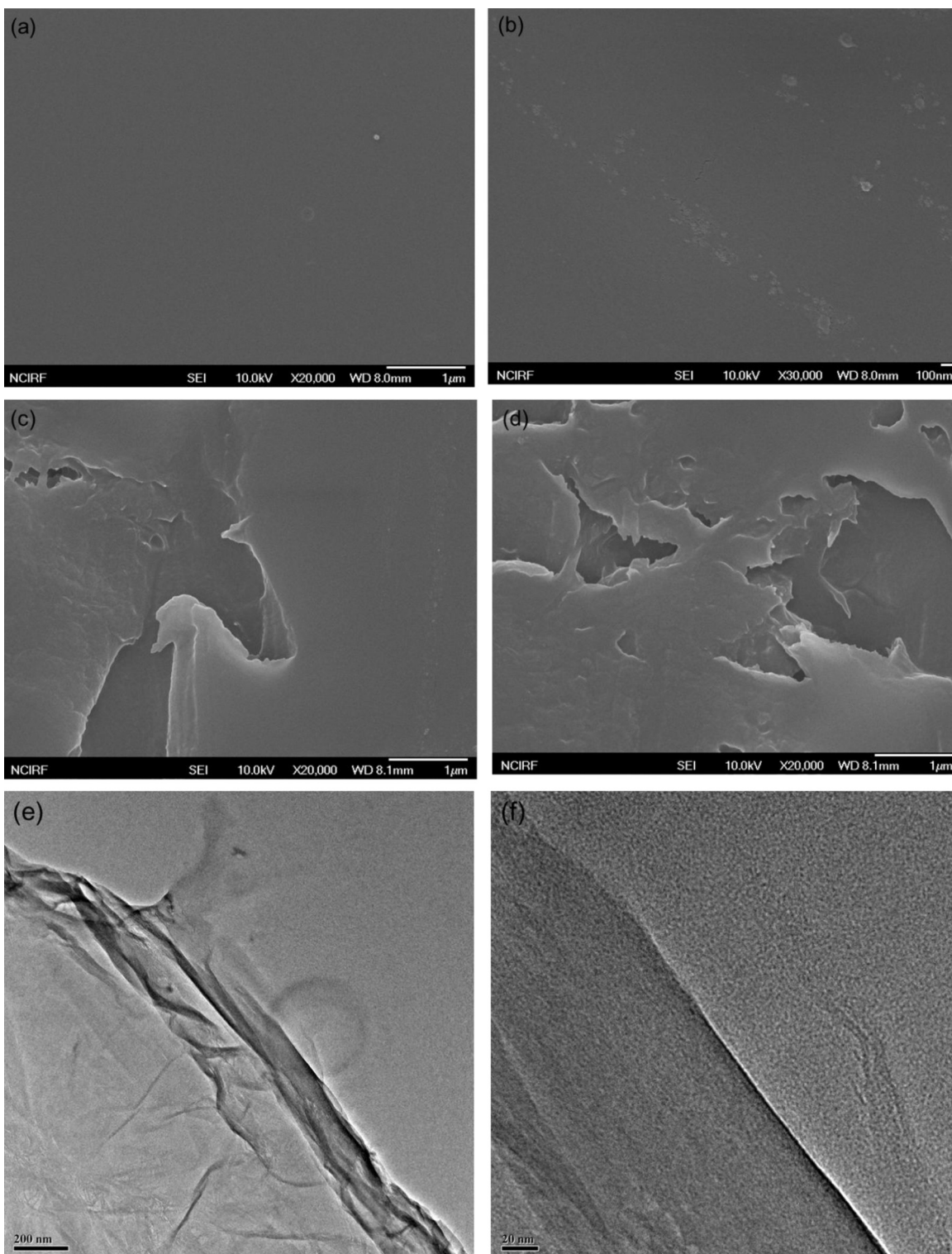
Fig. 5. SEM images of pure chitosan film (a and b), chitosan/graphene oxide bionanocomposite (c and d) and TEM images of chitosan/graphene oxide bionanocomposite (e and f).
