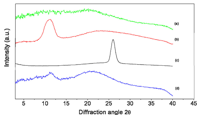
Fig. 4. XRD of pure chitosan film (a), pristine graphene oxide (b), graphite (c) and chitosan/graphene oxide bionanocomposite (d).
