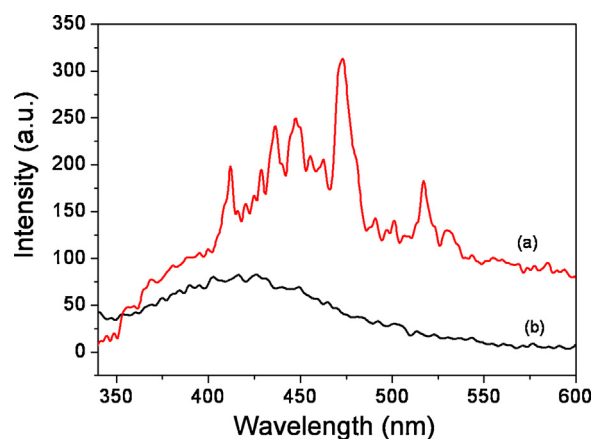
Fig. 8. PL spectra of pristine graphene oxide (a) and chitosan/graphene oxide (b) at excitation wavelength of 255 nm.
