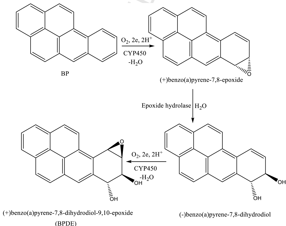
Scheme 1. Metabolism of BP by CYP450 yielding the carcinogenic benzo(a)pyrene-7,8-dihydrodiol-9,10-epoxide (BPDE).
