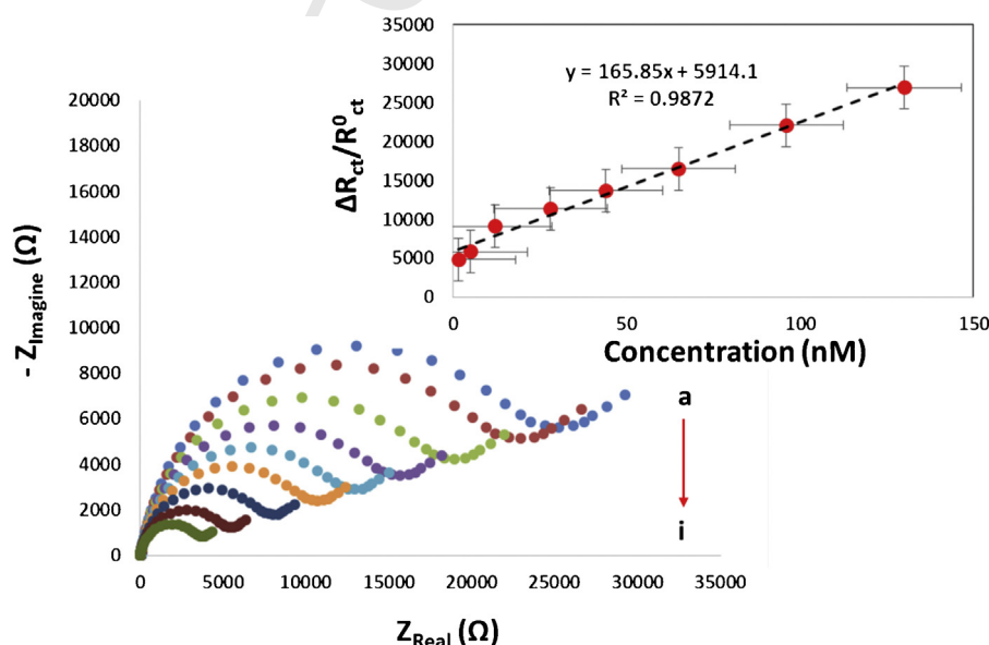
Fig. 5. The EIS curves of the DNA/HRP/SWCNTs-NA-IL/GCE in 5 mM [\text{Fe}(\text{CN})_6]^{3-/4-} solution containing 0.1 M KCl adjusted by the PBS (0.1 M, pH 5.5) after immersion for 10.0 min into several BP + \text{H}_2\text{O}_2 solutions. The solutions contain a constant concentration of \text{H}_2\text{O}_2 (2.0 mM), but different concentrations of BP including: (a) 0.0, (b) 1.5 nM, (c) 5.0 nM, (d) 12.0 nM, (e) 28.0 nM, (f) 44.0 nM, (g) 65.0 nM, (h) 96.0 nM, and (i) 130.0 nM. Inset: The corresponding calibration plot of \Delta R_{\text{ct}}/R_{\text{ct}}^0 versus different concentrations of BP.
