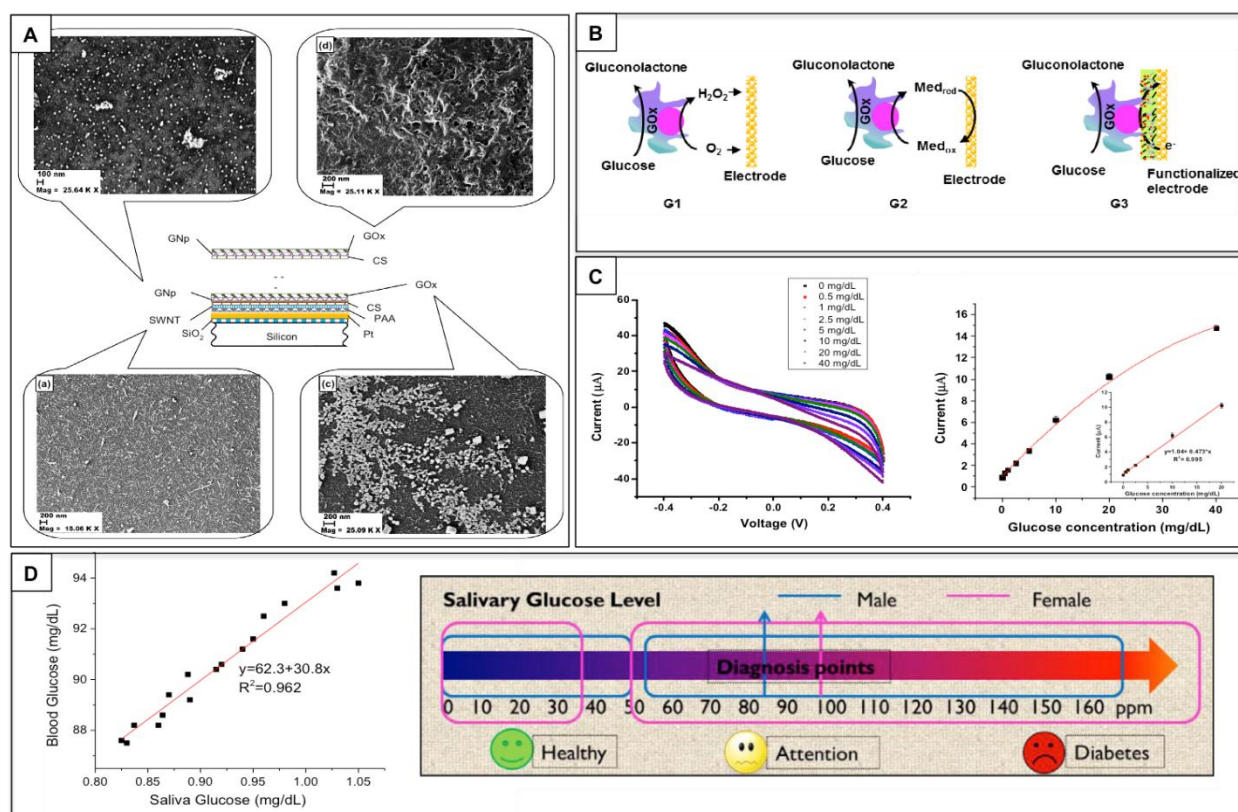
Fig. 2: (A) Cross-section of the functional layers on the sensor electrode and SEM images of one layer of SWNT (top left corner); one layer of SWNT/GNp (top right corner); PAA/SWNT/CS/GNp/GOx film (bottom left corner); PAA/SWNT/(CS/GNp/GOx) 3 (bottom right corner);) film on the sensor electrode surface. (B) A general scheme depicting the three enzymatic glucose detection mechanisms, presented as the first (G1), second (G2), and third (G3) generation glucose sensors. (C) Glucose sensing using the on-chip electrochemical sensing system S2D2 by cyclic voltammetry of Pt electrode modified with PAA/SWNT/ (CS/GNp/GOx) 3 layers obtained in 0–40 mg/dL glucose solutions with the voltage between WE and RE ranges from -0.4 V to 0.4 V at a scan rate of 50 mV/s; steady-state calibration curve of the PAA/SWNT/(CS/GNp/GOx) 3 functionalized Pt electrode at applied potential 0.2 V with linear detection range shown in the inset. Error bars = \pm standard deviation and n = 3 . (D) Correlation between blood glucose and saliva glucose of a healthy subject at fasting state; summarized saliva glucose levels indicating individuals' health conditions from literature [56].
