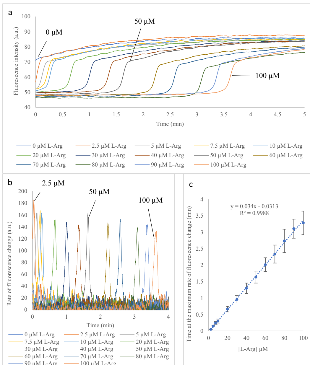
Fig. 6. Time-course fluorescence measurements on 265Cf in different concentrations of L-Arg in PBS solution. L-Arg in different concentrations (0–100 μM) was mixed with (a) 265Cf. (b) The rates of the fluorescence changes at different concentrations of L-Arg. (c) The linear relationship between the time at the maximum rate of the fluorescence change and the L-Arg concentration.
