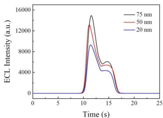
Figure S14. The ECL intensity of the Au@21.5 nm SiO 2 -based MASNEs with different AuNPs sizes in 0.1 M PBS (pH=9) buffer containing 20 \mu M Ru(bpy) 3 2+ and 0.1 mM tripropylamine (TPrA). Related to Figure 3.
