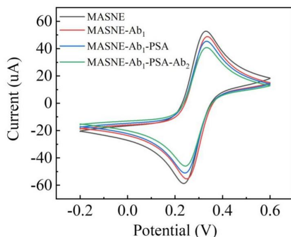
Figure S17. Cyclic voltammograms (in 2 mM \text{K}_3\text{Fe}(\text{CN})_6 solution, sweep rate 50 mV/s) for the ECL sensing platform during the fabrication. Compared with the bare MASNE, the peak current decreases after every modification step because of the poor conductivity of the biomolecules and \text{Ru}@\text{SiO}_2 . Related to Figure 5.
