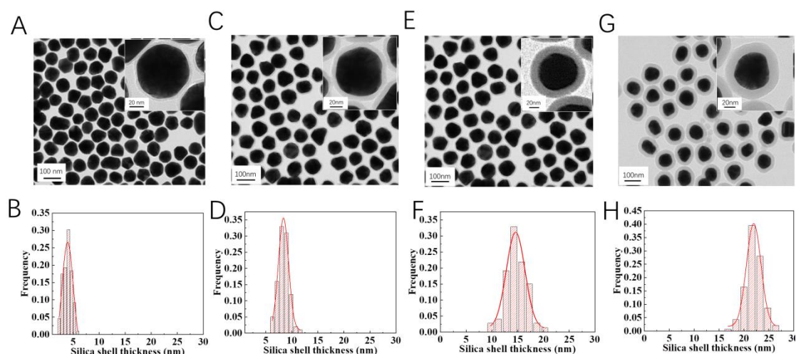
Figure S1. TEM images and silica shell thicknesses distributions of 75 nm Au@SiO 2 NPs. (A-B) 75 nm Au@4.0 ± 0.8 nm SiO 2 NPs, (C-D) 75 nm Au@8.4 ± 1.1 nm SiO 2 NPs, (E-F) 75 nm Au@14.9 ± 2.0 nm SiO 2 NPs, (G-H) 75 nm Au@24.6 ± 2.7 nm SiO 2 NPs. Data are represented as mean ± TEM. Related to Figure 2.
