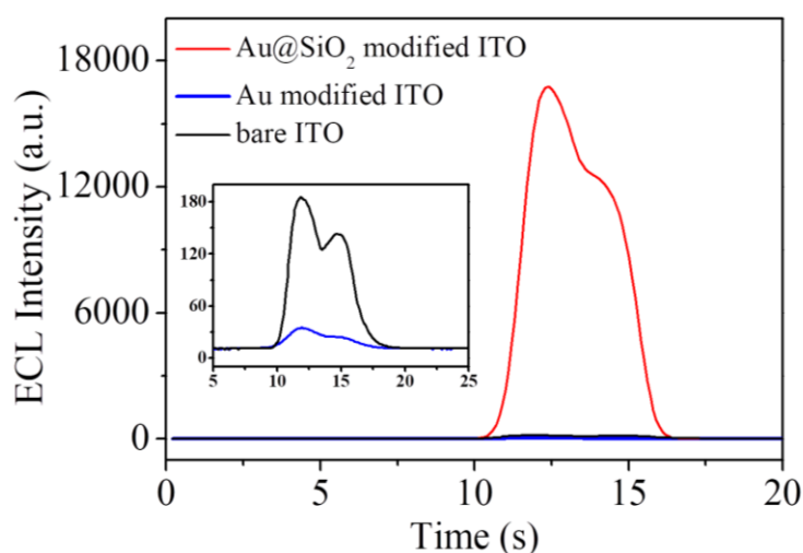
Figure S6. The comparison of ECL intensity between 75nm Au@21.5 nm SiO 2 NPs and 75 nm AuNPs fabricated ECL electrodes using Ru@SiO 2 as luminophore. Inset: enlarged image of ECL intensity of Au modified ITO and bare ITO electrode. Related to Figure 3.
