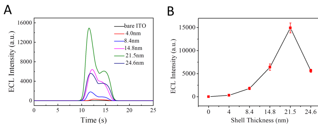
Figure S5. ECL intensity of the 75 nm Au@ SiO 2 modified MASNE with different silica shell thicknesses (0.1 M PBS solution (pH=9) containing 20 \mu\text{mol L}^{-1} Ru(bpy) 3 2+ and 0.1 mmol L -1 TPrA). Related to Figure 3.
