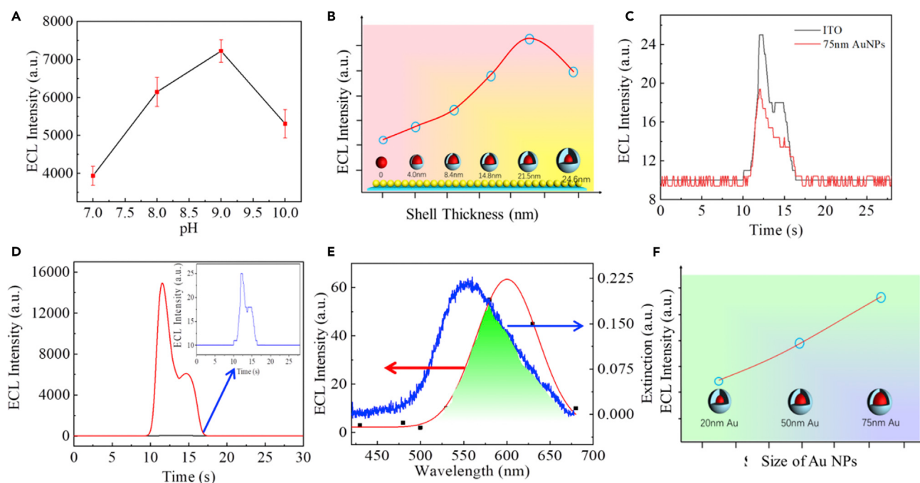
Figure 3. Performance of MASNE in \text{Ru}(\text{bpy})_3^{2+} -Based Plasmonic ECL System
