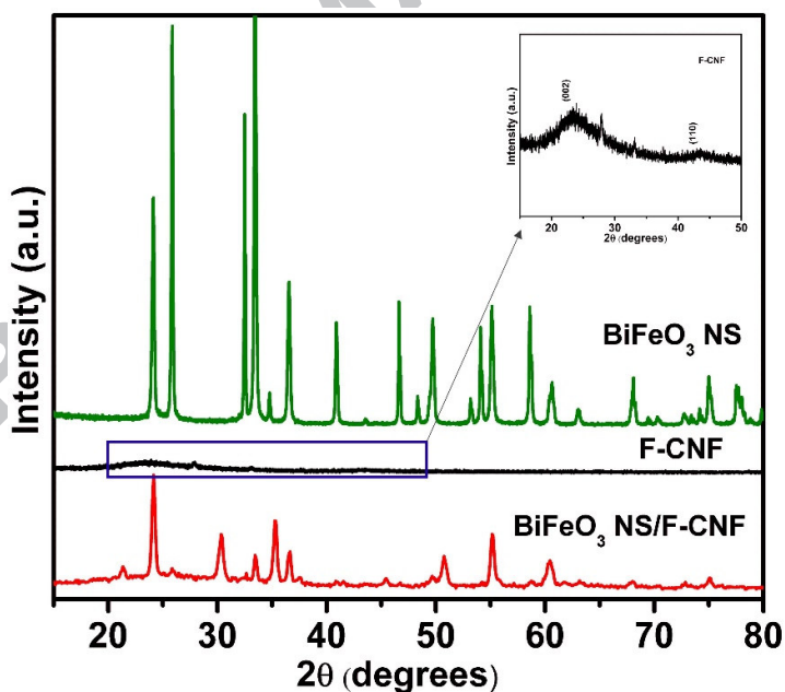
Fig. 3 XRD pattern of \text{BiFeO}_3 NS, F-CNF and \text{BiFeO}_3 NS/F-CNF nanocomposite.
