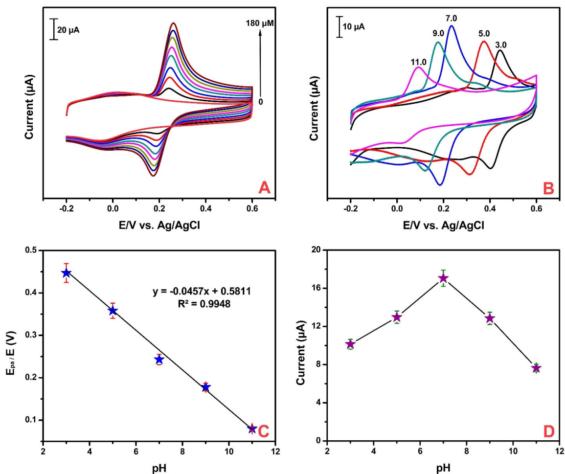
Fig. 8 (A) CV curve of BiFeO 3 NS/F-CNF/GCE by varying the concentration of CC (0-180 μM) in N 2 saturated 0.05 M PBS (pH 7) at scan rate of 50 mVs -1 , (B) The effect of pH (3-11) of the electrolyte solution at BiFeO 3 /F-CNF/GCE with presence of CC (100 μM). (C) The corresponding calibration pH vs. plots of oxidation peak potential and (D) pH vs. oxidation peak currents.
