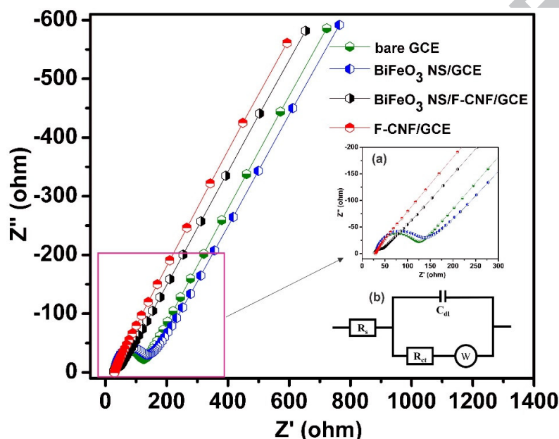
Fig. 6 EIS curve of bare GCE, BiFeO 3 NS, F-CNF and BiFeO 3 /F-CNF in 5 mM of [Fe(CN) 6 ] 3-/4- contain 0.1 M of KCl in the frequency range from 0.1 Hz to 100 kHz. Inset: (a) High magnified image of EIS curves (b) Randles circuit model.
