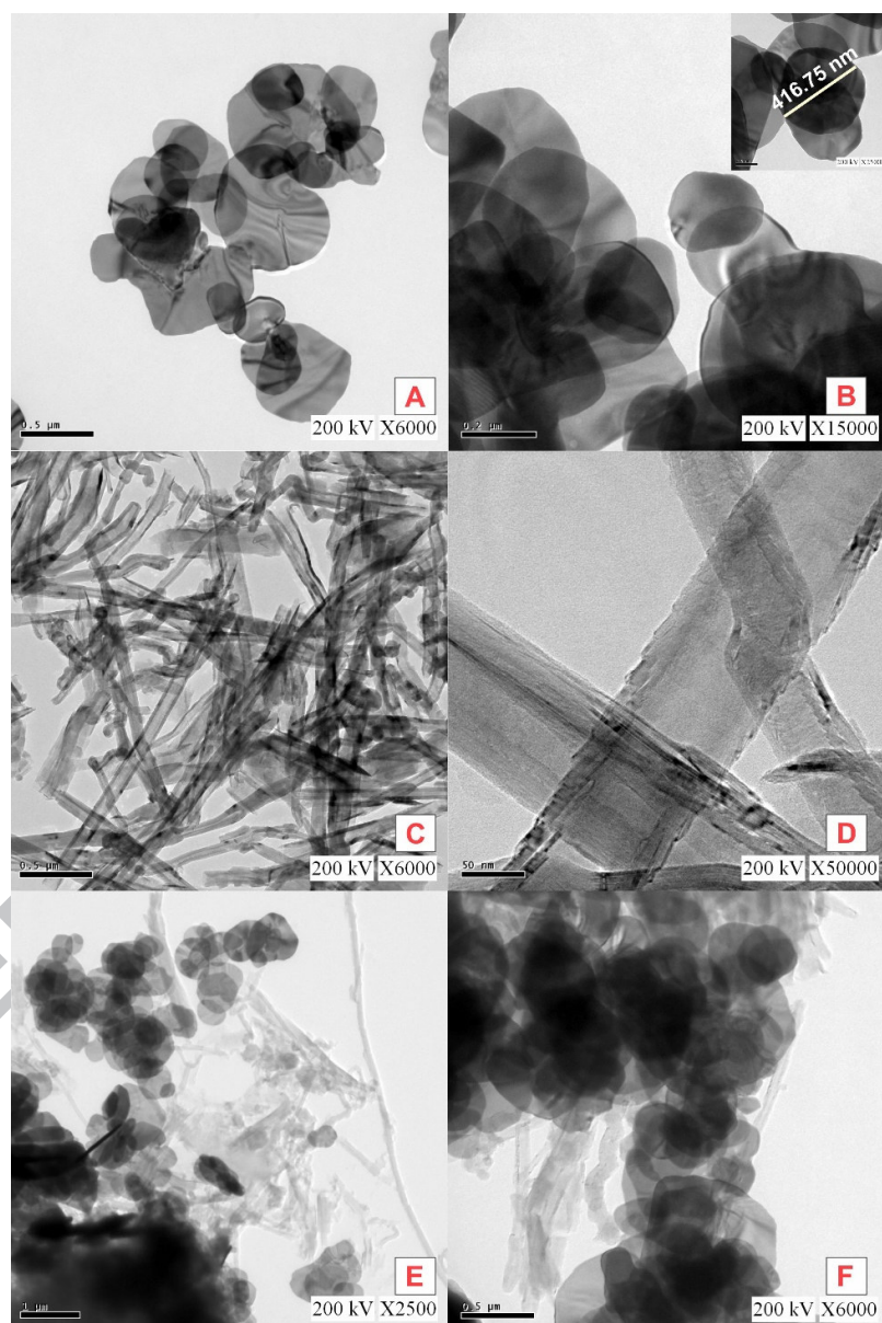
Fig. 2 TEM images of (A, B) \text{BiFeO}_3 NS (C, D) F-CNF and (E, F) \text{BiFeO}_3 NS/F-CNF.
