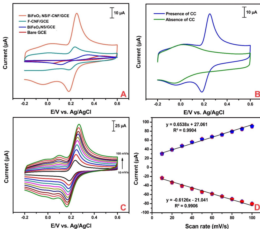
Fig. 7 (A) CV behavior of bare GCE, BiFeO 3 NS/GCE, F-CNF/GCE and BiFeO 3 NS/F-CNF/GCE in the presence of CC (100 μM) containing N 2 saturated 0.05 M PBS (pH 7) at a scan rate of 50 mVs -1 , (B) Presence and absence of CC (100 μM) at BiFeO 3 NS/F-CNF/GCE in N 2 saturated 0.05 M PBS (pH 7) at scan rate of 50 mVs -1 , (C) CV curve of the BiFeO 3 NS/F-CNF/GCE in N 2 saturated 0.05 M pH 7.0 containing CC (100 μM) by varying scan rate from 10 to 100 mVs -1 , (D) The calibration plot for scan rate vs. oxidation and reduction peak current.
