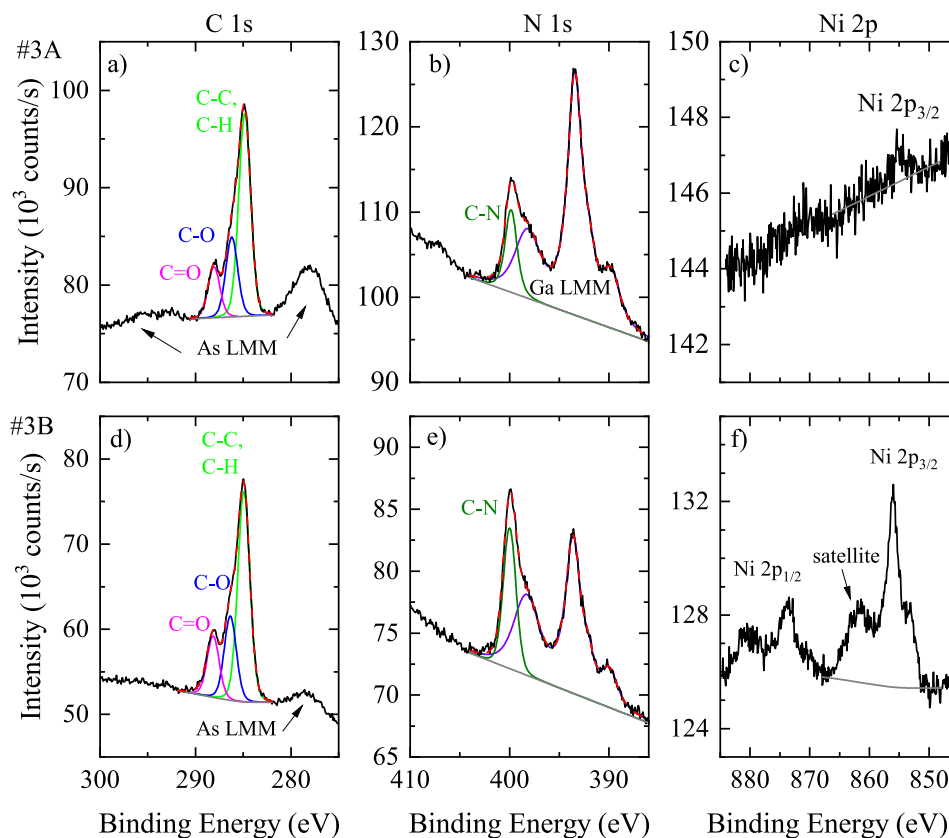
Fig. 4. XPS high resolution scans for C 1s (a, d), N 1s (b, e) and Ni 2p (c, f) regions for two distinct areas of sample #3, A (top row: a–c) and B (bottom row: d–f), where A was exposed to UV light while covered with neutravidin solution, and B was exposed to UV light while covered with Ni-ENSA solution. The background baseline is shown in grey. Fitted components for C 1s include C – C and C – H (green), C – OH, C – O – C and C – N (blue), C = O (magenta) and O – C = O (cyan), respectively, with the dashed red line being their sum; this region is overlapped by As LMM Auger peaks (not fitted). The N 1s region includes the fit for C – N (green), overlapped by Ga LMM Auger peaks (also fitted), with the dashed red line being their sum. The Ni 2p 3/2 peak region, overlapped by a satellite [37], was used for quantification of this element.
