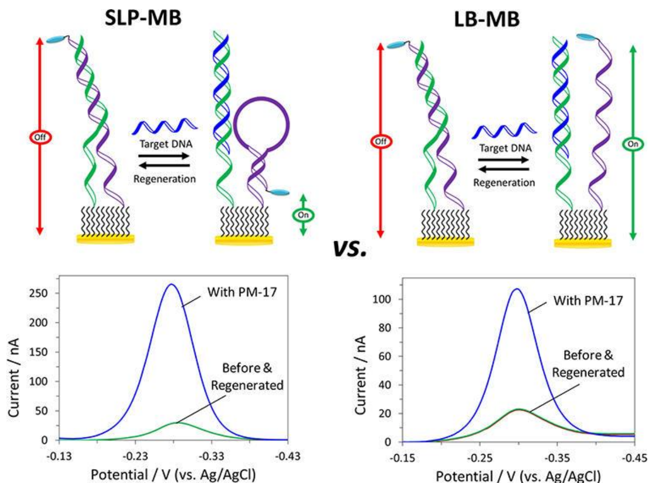
Figure 3. Hybridization induced conformational and dynamic DNA signal transduction mechanisms. The stem-loop methylene blue terminated probe (SLP-MB) is conformationally brought to the surface when displaced by the target ssDNA, while the linear methylene blue terminated probe (LB-MB) is dynamically brought to the surface when displaced by target ssDNA. Both restore the amperometric response. Reprinted with permission from Ref. [37]. Copyright 2013 American Chemical Society.
