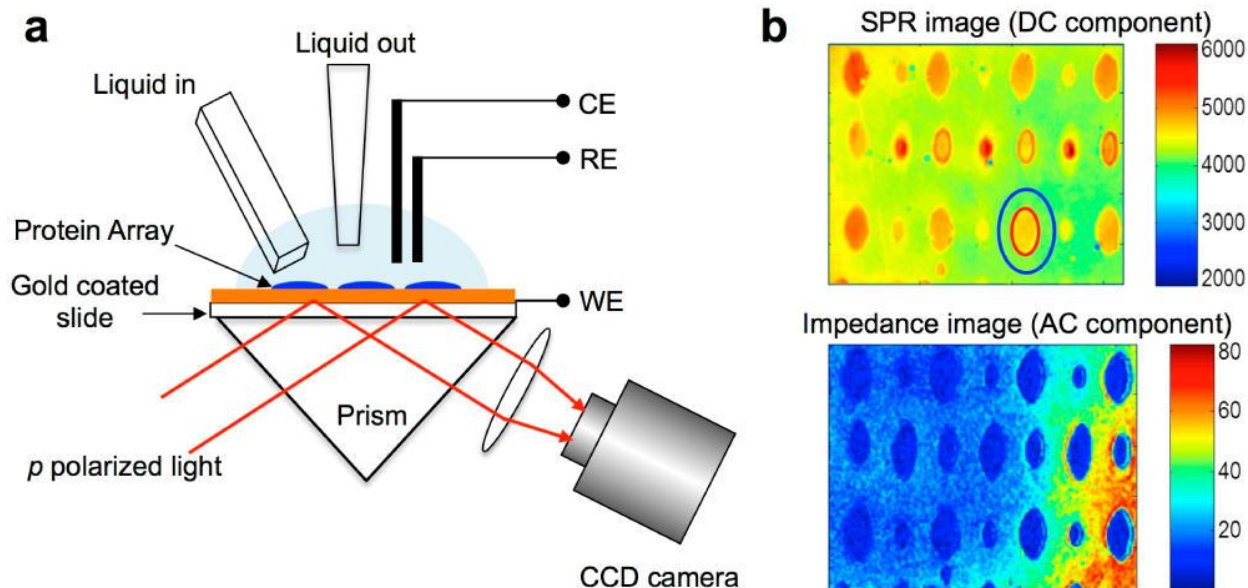
Figure 7. Working schematic of EIS-SPR and expected results. (a) Experimental setup for EIS-SPR imaging. Counter electrode and reference electrode are in the flow medium, while the working electrode is the SPR sensor chip. (b) Representative results, where the conventional SPR image is the DC component of the response, and the impedance can be imaged through the AC component. Reprinted with permission from Ref. [112]. Copyright 2014 American Chemical Society.
