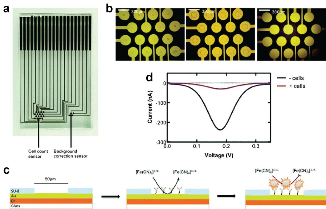
Figure 1. Electrochemical detection of prostate cancer cells with aperture sensor array. (a) Photograph of multiplexed chip. (b) Individual sensing areas of varying size. (c) Detection scheme utilizing redox reporter in solution. (d) Differential pulse voltammograms before and after binding of cells. Adapted from Ref. [9] with permission of The Royal Society of Chemistry.
