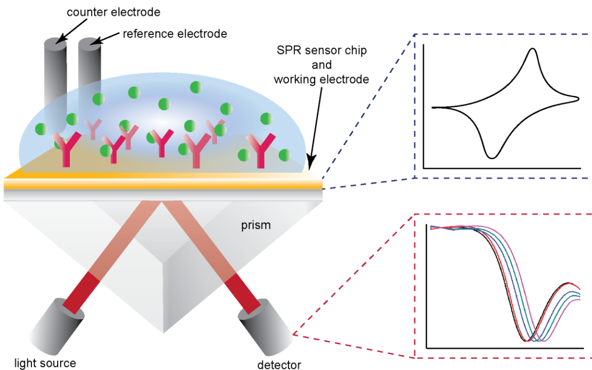
Figure 6. Surface plasmon resonance setup with integrated electrochemical equipment. The SPR sensor chip functions for reflectivity measurements, and as the working electrode. Counter and reference electrodes are generally placed in the flow medium.
