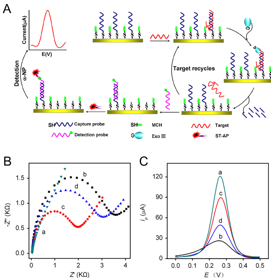
Fig. 8. (A) Schematic illustration of the electrochemical DNA biosensor for the detection of Enterobacteriaceae bacteria. (B) EIS, and (C) SWVs for (a) bare electrode, (b) capture DNA modified electrode, (c) capture DNA modified electrode after the reaction with target DNA and Exo III, and (d) further reaction with detection probe. Reprinted from [47] with permission: Copyright © 2013 Elsevier B.V.
