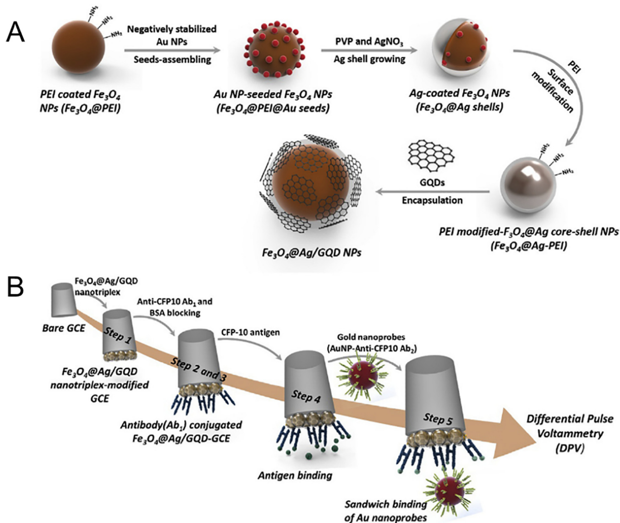
Fig. 4. Schematic illustration of (A) the preparation of \text{Fe}_3\text{O}_4@\text{Ag}/\text{GQD} nanoparticles and, (B) modification of GCE electrodes for the detection of Mycobacterium tuberculosis using a sandwich-type electrochemical immunosensor. Reprinted from [32] with permission: Copyright © 2018 Elsevier B.V.
