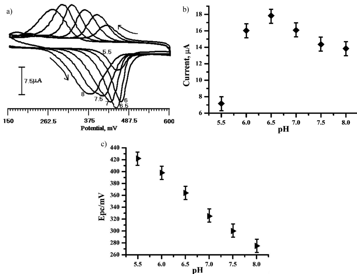
Fig. 8 – (a) Cyclic voltammograms obtained at the PGMCPPE in 0.2 M PBS in pH values, (a) 5.5 (b) 6 (c) 6.5 (d) 7 (e) 7.5 (f) 8 containing IC ( 1 \times 10^{-4} M). (b) Plot of anodic peak current vs. pH (5.5–8.0) of IC ( 1 \times 10^{-4} M) at the PGMCPPE. (c) Plot of E_{pc} vs pH for IC.
