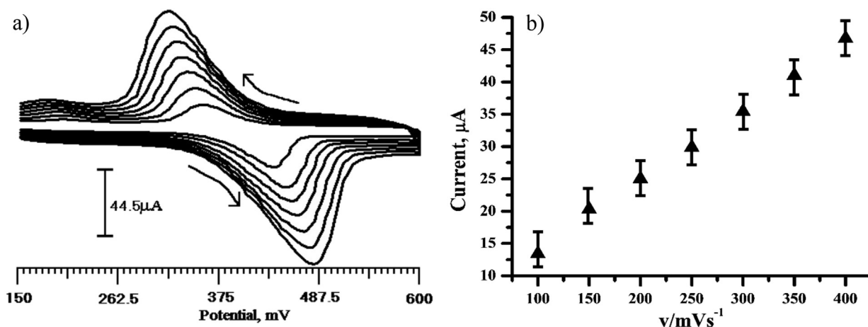
Fig. 7 – (a) Cyclic voltammograms of IC ( 1 \times 10^{-4} M) at the PGMCPPE in pH 6.5 PBS at various scan rates. From: 100, 150, 200, 250, 300, 350 and 400 mV/s. (b) Plot of the peak current of IC as a function of the scan rate.
