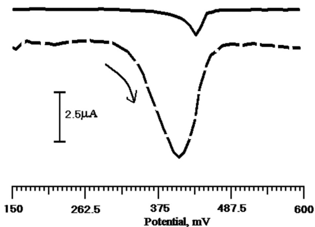
Fig. 6 – DPVs of a solution containing IC ( 1 \times 10^{-4} M) in 0.2 M PBS (pH 6.5) at the BCPE (solid line), the PGMCPPE (dashed line).
