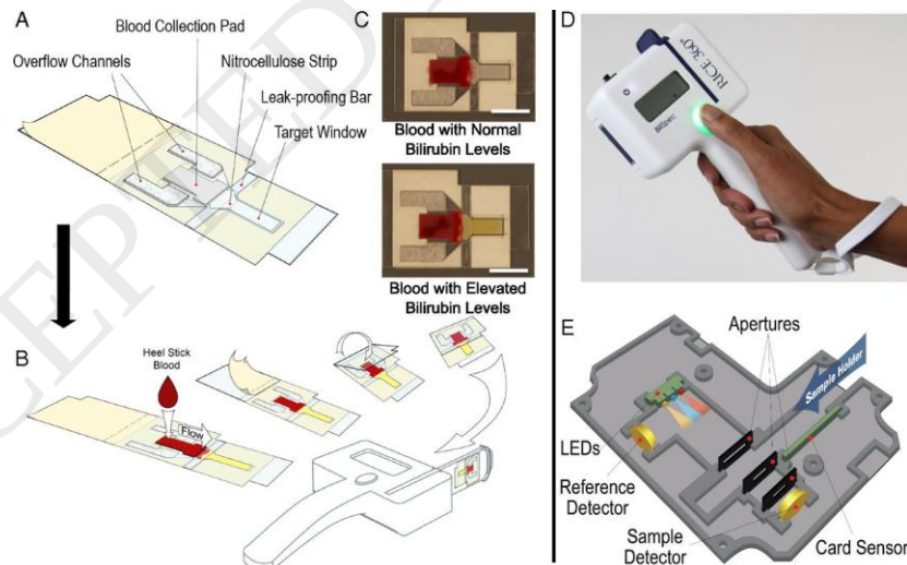
Figure 5 BiliSpec lateral flow card and reader. (A) Diagram of the lateral flow card components. To use the card, blood is applied to the collection pad, protective paper is removed from the adhesive-coated acetate, and the card is folded to seal blood inside. (B) Plasma flows down to the distal tip of the card before being inserted into the reader for measurement. (C) Representative photographs of sealed lateral flow cards following application of blood with normal and elevated TSB levels. (Scale bar, 1 cm.) (D) Photograph of the hand-held reader. (E) Diagram illustrating the internal optical and electronic layout of the reader [100].
