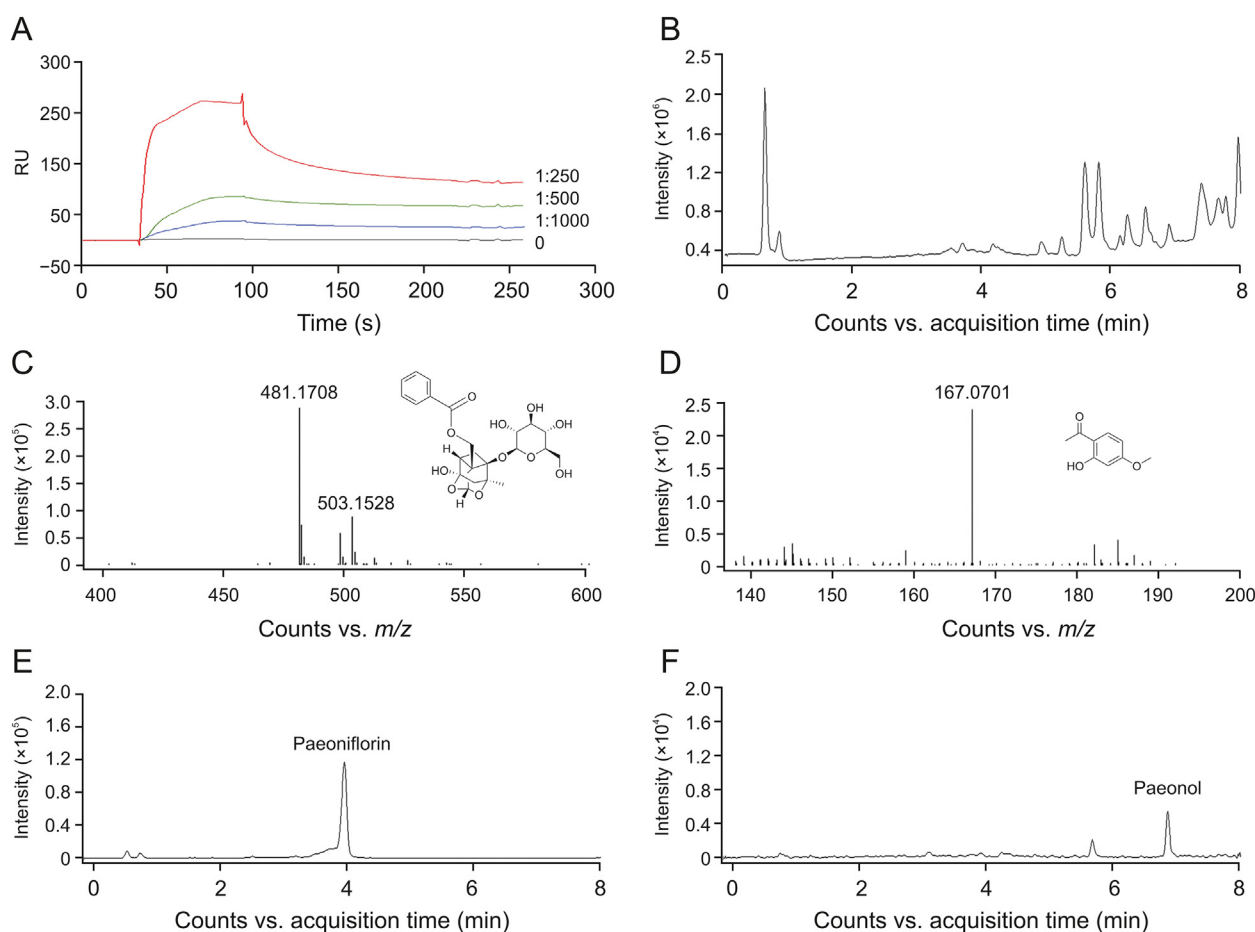
Fig. 2. Recovery and identification of TNF-R1-bound ingredients from Radix Paeoniae Alba (RPA). (A) RPA extraction displayed binding activity to TNF-R1 in a dose-dependent manner. (B) Total ion chromatography (TIC) of the recovered sample. (C) Mass spectrometry and chemical structure of paeoniflorin identified from the recovered sample. (D) Mass spectrometry and chemical structure of paeonol identified from the recovered sample. (E) TIC of paeoniflorin standard. (F) TIC of paeonol standard.
