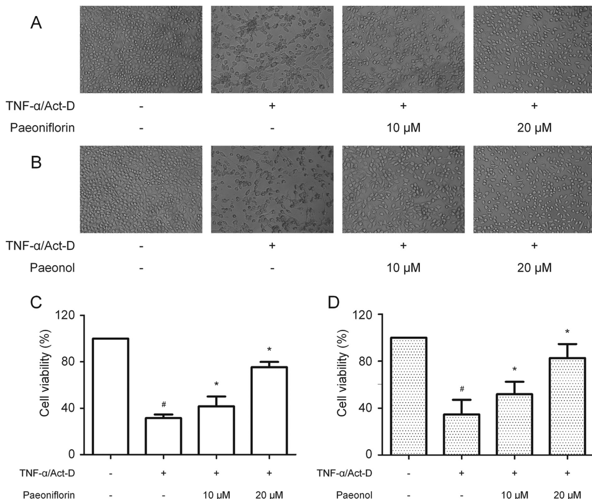
Fig. 6. Effects of paeoniflorin and paeonol on cell viability of L929 cells. L929 cells were incubated with the indicating concentrations of paeoniflorin or paeonol in the absence or presence of TNF- \alpha and actinomycin D (Act-D) for 48 h. (A and B) Representative cell views of each group. (C and D) Cell viability was determined by CCK8 assay. Data presented are means \pm SD of three independent experiments. # P < 0.05 versus non-stimulated control, * P < 0.05 versus TNF- \alpha /Act-D alone by student t -test.
