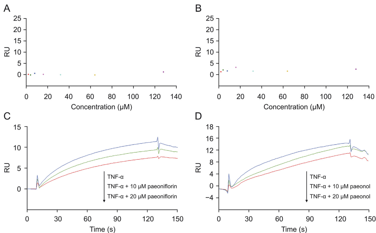
Fig. 4. Competition between active candidates and TNF- \alpha analyzed by SPR competition assay. (A) A serial concentration of paeoniflorin tested on TNF- \alpha sensor surface showed there was no specific binding. (B) A serial concentration of paeonol tested on TNF- \alpha sensor surface showed there was no specific binding. (C) Competition assay of paeoniflorin and TNF- \alpha revealed that paeoniflorin could block the binding of TNF- \alpha towards TNF-R1 in a concentration-dependent manner. (D) Competition assay of paeonol and TNF- \alpha revealed that paeonol could block the binding of TNF- \alpha towards TNF-R1 in a concentration-dependent manner.
