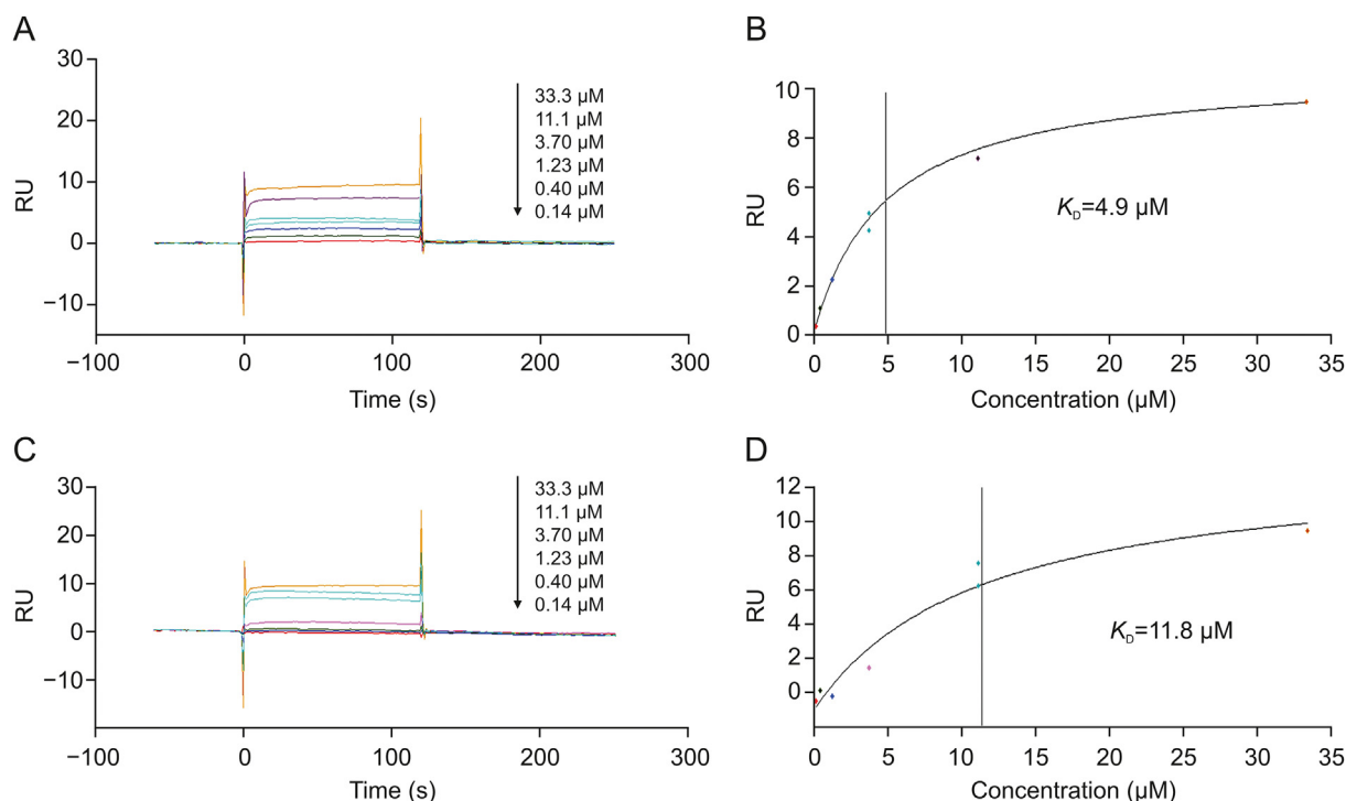
Fig. 3. Affinities of the bioactive candidates towards TNF-R1 determined by surface plasmon resonance (SPR) affinity assay. (A) Sensorgrams of serial concentrations of paeoniflorin (0–33.3 μM). (B) Affinity constant of paeoniflorin. (C) Sensorgrams of serial concentrations of paeonol (0–33.3 μM). (D) Affinity constant of paeonol.
