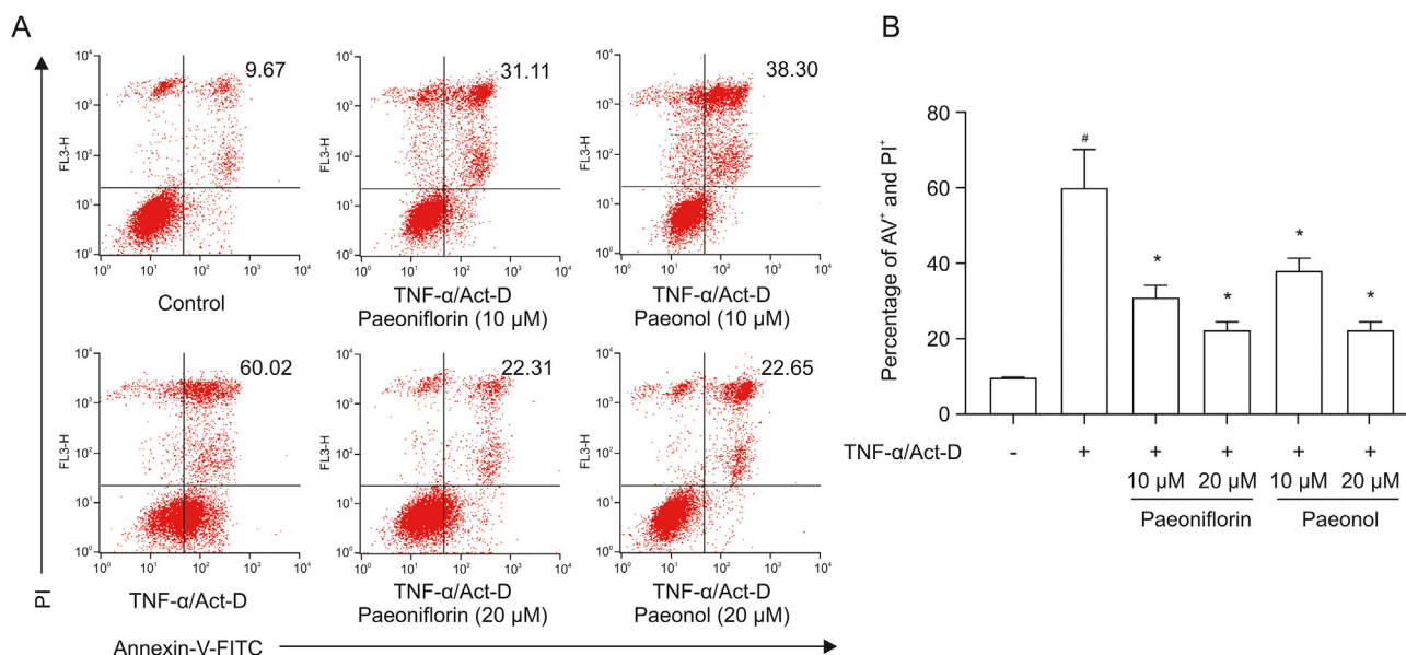
Fig. 7. Effects of paeoniflorin and paeonol on apoptosis of L929 cells. L929 cells were incubated with the indicated concentrations of paeoniflorin or paeonol in the absence or presence of TNF- \alpha and Act-D for 48 h. (A) The cells labeled with Annexin-V-fluorescein isothiocyanate (FITC) and propidium iodide (PI) were analyzed by flow cytometry. (B) The percentage of cell apoptosis was calculated. # P < 0.05 versus non-stimulated control, * P < 0.05 versus TNF- \alpha /Act-D alone by Student's t -test.
