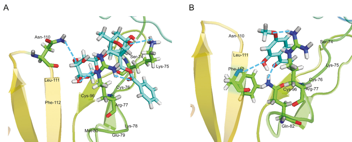
Fig. 5. The interplay between TNF-R1 and (A) paeoniflorin or (B) paeonol. Paeoniflorin and paeonol had the best poses with subdomain 1 of TNF-R1.
