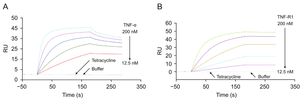
Fig. 1. The bioactivity of the sensor chip was characterized by positive and negative controls after protein immobilization. (A) For tumor necrosis factor receptor type 1 (TNF-R1) sensor chip, tumor necrosis factor- \alpha (TNF- \alpha ) could bind to TNF-R1 specifically. (B) For TNF- \alpha sensor chip, TNF-R1 could bind to TNF- \alpha specifically.
