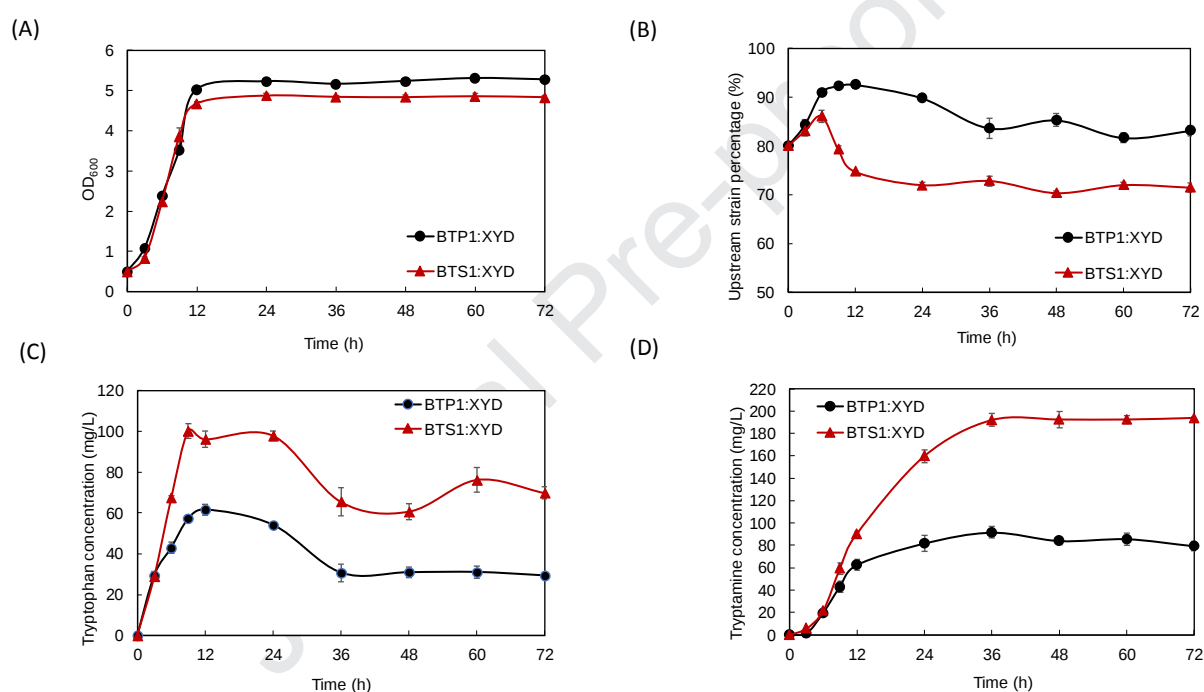
Fig. 6 Shake flask cultivation of the BTP1:XYD and BTS1:XYD co-cultures for the tryptamine bioproduction. Time profiles of (A) overall co-culture cell density, (B) upstream strain percentage, (C) accumulation of the pathway intermediate tryptophan and (D) concentration of tryptamine were derived from triplicate shake flask runs. Error bars represent standard errors of the experimental results.
