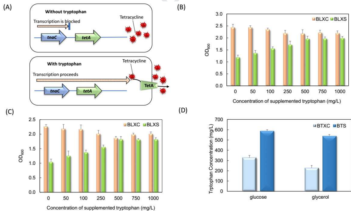
Fig. 3 Construction and characterization of the tnaC-tetA cell selection system. (A) Scheme of the tnaC-tetA cell selectin mechanism. The presence of tryptophan decides whether the tetA gene
