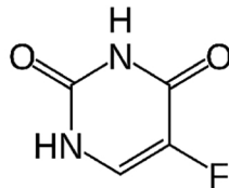
Fluorouracil
