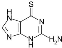
Thioguanine
