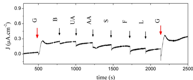
Fig. 7. Amperometric responses of ITO/(GPDDA/GPSS) 1 /(GPDDA/GOx) 2 electrode at -0.3 V vs SCE upon additions of 100 \mu\text{L} of 20 \text{mmol}\cdot\text{L}^{-1} of glucose (G), buffer (B), uric acid (UA), ascorbic acid (AA), lactose (L), sucrose (S) and fructose (F) in 10 \text{mmol}\cdot\text{L}^{-1} phosphate buffer (pH 6.3).
