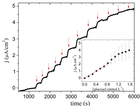
Fig. 6. Amperometric response of ITO/(GPDDA/GPSS) 1 /(GPDDA/GOx) 2 electrode at -0.3 V vs SCE upon successive addition of 100 \mu\text{L} of glucose in 10 \text{mmol}\cdot\text{L}^{-1} phosphate buffer (pH 6.3). Inset: Analytical curve with linear range from 0.14 to 0.95 \text{mmol}\cdot\text{L}^{-1} .
