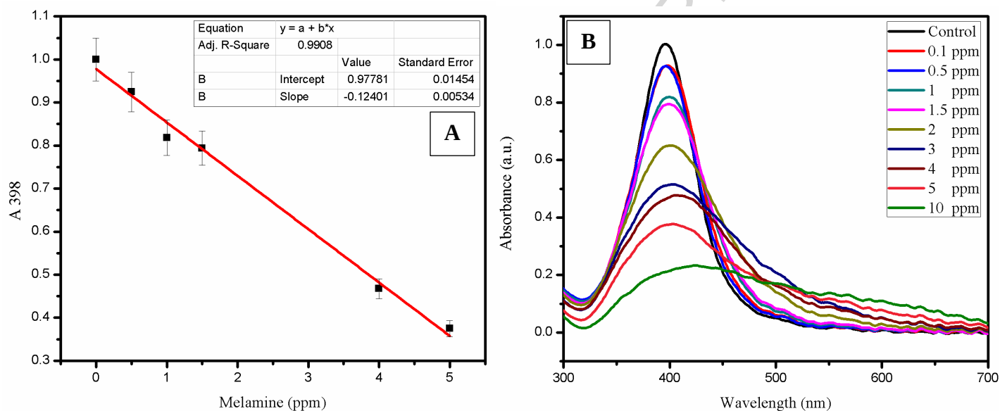
Figure 3 A) The calibration curve between absorbance at 398 nm and concentration of melamine for the calculation of linearly dependent coefficient. B) UV-Vis absorption spectra of interference green synthesized Ag with different concentration of melamine (0.1 to 10 ppm, Control: 0 ppm).
