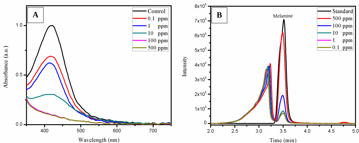
Figure 5 A) UV-Vis absorption spectra of Ag nanoparticles synthesized with different concentrations of melamine (0.1-500 ppm) from pre-processed milk B) HPLC chromatograms obtained after spiking milk with different concentrations of melamine; 0.1-500 ppm (Standard: 1000 ppm melamine in water, Column: C18, UV detection: 240 nm, Injection volume: 3 \mu L, Mobile phase; Acetonitrile: H 2 O - 70:30, Flow rate: 0.7 mL/min).
