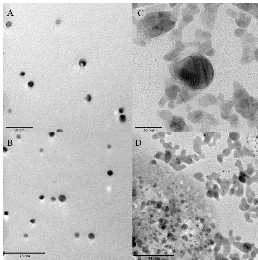
Figure 4 Different scales of TEM images of interference green synthesis of Ag nanoparticles with and without melamine (A, B – Without melamine; C, D – With 100 ppm melamine; Scale: A, C – 50 nm; B, D – 75 nm).
