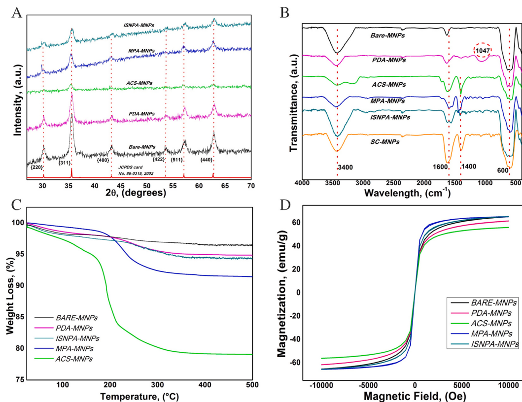
Fig. 5. Different characterization results for bare and coated MNPs (polydopamine, (PDA), citric acid (ACS), mercaptopropionic acid (MPA), isonipecotic acid (ISNPA)@MNPs), and sodium citrate (SC@MNPs) employing: (A) X-ray diffraction analysis, (B) Fourier transform infrared spectroscopy, (C) Thermogravimetric analysis, and (D) Vibrating sample magnetometer analysis.
