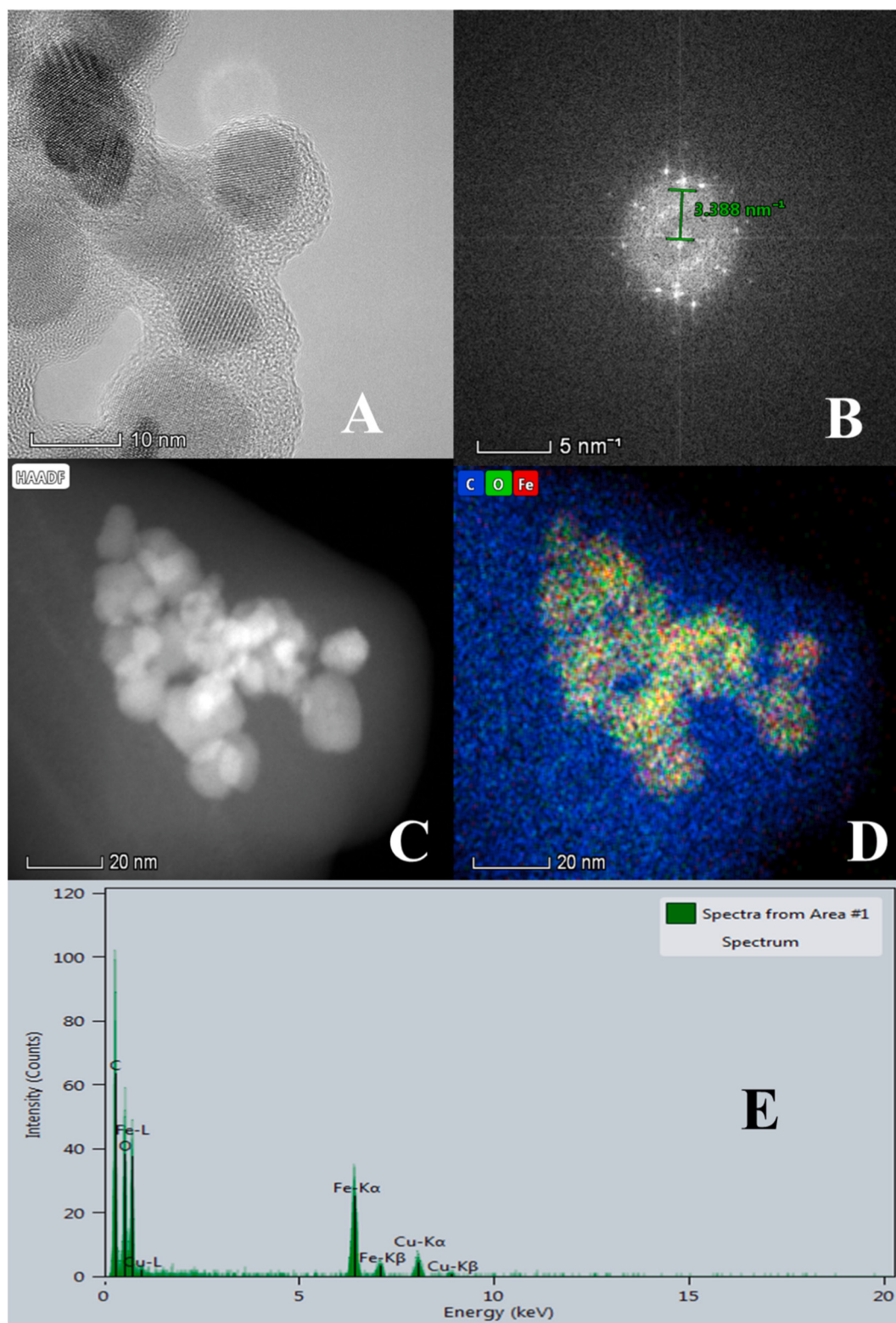
Fig. 4. Transmission electron microscopy (TEM) analysis of polydopamine (PDA)@MNPs. A) TEM micrograph of PDA@MNPs taken at HREM mode, B) Digital Diffraction Pattern (DDP) built from A, C) TEM micrograph of a MNPs cluster taken at HAADF mode, D) Compositional mapping from image C and E) EDS spectrum of image in micrograph C.
