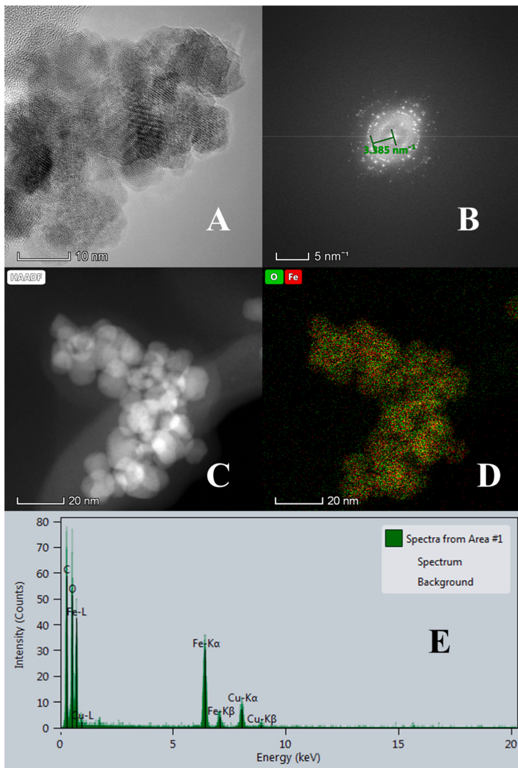
Fig. 3. Transmission electron microscopy (TEM) analysis of bare MNPs. A) TEM micrograph of MNPs taken at high resolution electron microscopy (HREM) mode, B) Digital Diffraction Pattern (DDP) built from A. C) TEM micrograph of a MNPs cluster taken at high-angle annular dark-field imaging (HAADF) mode, D) Compositional mapping from image C, and E) energy-dispersive X-ray spectroscopy (EDS) spectrum of image in micrograph C.
