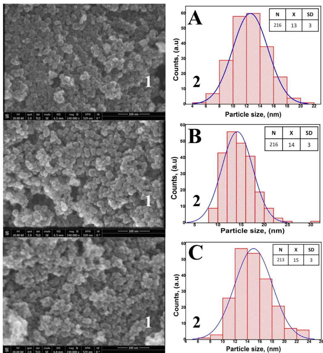
Fig. 1. Scanning electron microscopy (SEM) images of magnetic nanoparticles (MNPs) synthesized at different values of amplitude and 1 min of time. A.1) 40% B.1) 50% and C.1) 60%. Corresponding histograms and statistical charts are shown for each of them in A.2), B.2) and C.2), respectively. (N: counts, X: average size, SD: standard deviation).
