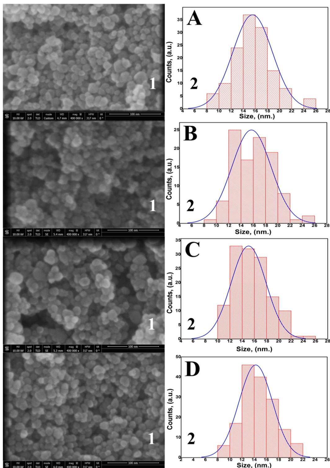
Fig. 2. SEM images of different functionalized MNPs synthesized at amplitude 40% and 1 min of time. A.1) polydopamine (PDA)@MNPs, B.1) citric acid (ACS)@MNPs, C.1) mercaptopropionic acid (MPA)@MNPs, and D.1) isonipecotic acid (ISNPA)@MNPs. Corresponding histograms and statistical charts are shown for each of them in A.2), B.2), C.2) and D.2), respectively. (N: counts, X: average size, SD: standard deviation).
