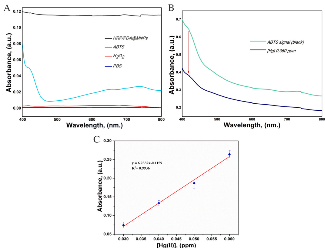
Fig. 6. (A) Absorbance spectra of different components ([horseradish peroxidase/polydopamine (HRP/PDA)@MNPs]: 0.25 mg/mL, [ABTS]: 0.3 mg/mL, [hydrogen peroxide (H 2 O 2 )]: 0.3% v/v, and [phosphate buffer solution (PBS)]: 0.1 M at pH 6. (B) Reduction of the ABTS signal due to irreversible inhibition of HRP enzyme by mercury. (C) Calibration curve built from the enzymatic inhibition study, measuring absorbance ( n = 3 ) at wavelength 417 nm.
