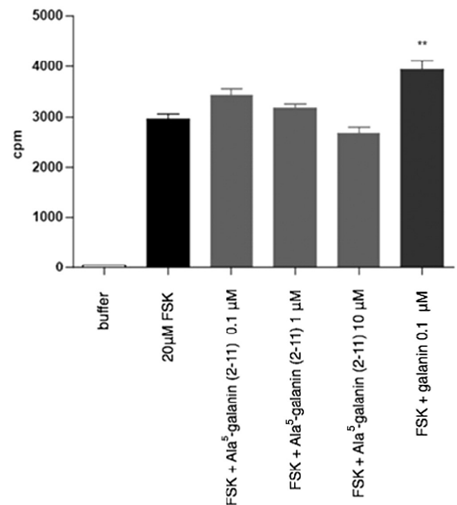
Fig. 2. Signal transduction using cyclic adenosine-monophosphate stimulation. Cyclic adenosine-monophosphate, cAMP, production was measured radiometrically. Ala 5 -galanin (2–11) did not significantly stimulate cAMP production in SH-SY5Y cells stably expressing human GAL 2 R. Full-length human galanin (0.1 \mu M) together with forskolin (FSK) were used as control. Data shown are mean values of triplicates \pm SEM of one experiment. **p-Value \leq 0.01 , ANOVA Bonferroni's multiple comparison test.
