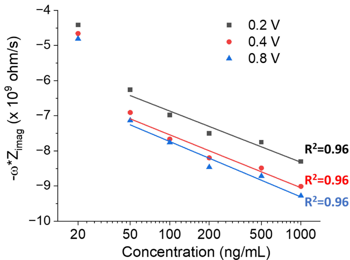
Figure 5 –. Correlation between -\omega * Z_{imag} and concentration of NPY in aCSF at 0.2 V, 0.4 V, and 0.8 V, showing a linear correlation in all of them with R^2=0.96 .
