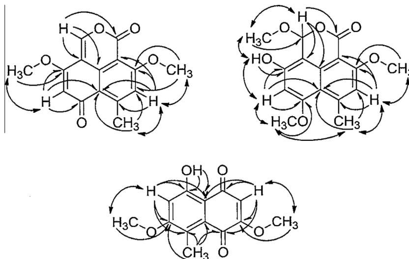
Fig. 1. Selected HMBC (→) and NOESY (↔) correlations of 1–3 .
