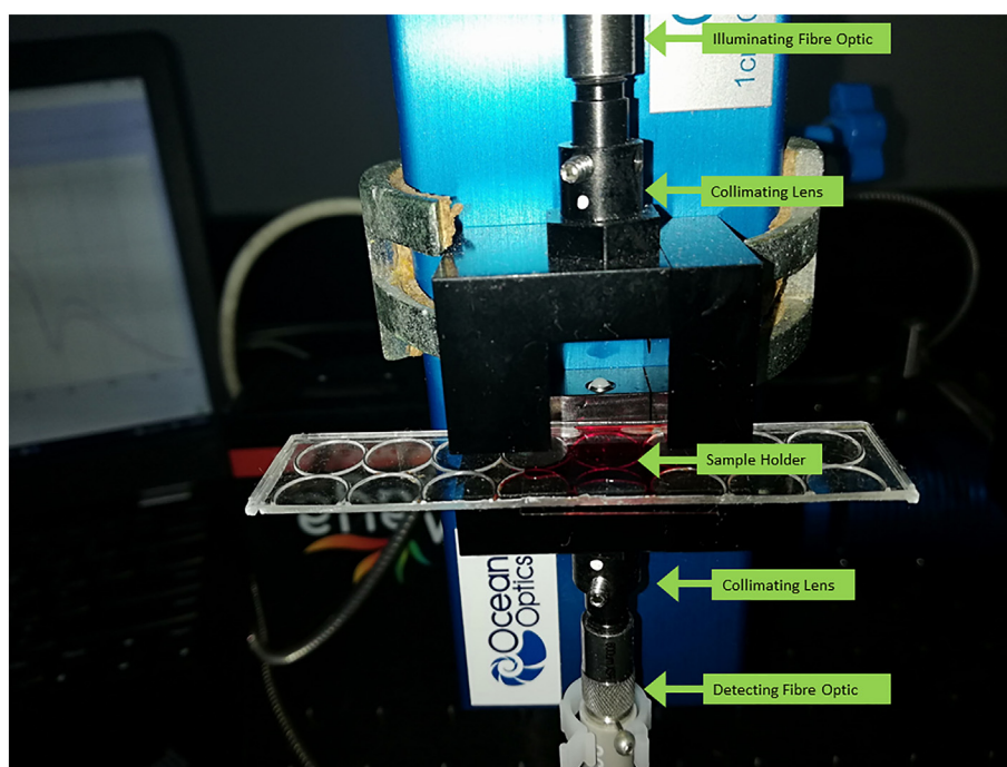
Fig. 2.3. Sample holder set-up, comprising an inverted 96 well plate cover and cover slip, for measuring the UV-Vis-NIR spectral absorbance of control, Plasmodium and Trypanosoma infected mouse blood samples, with a 0.4 mm ( \pm 0.1 ) optical path length and approximately 22.5 \mu l volume.
