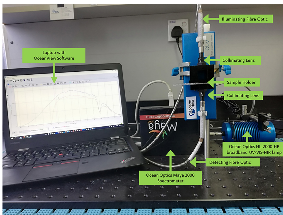
Fig. 2.2. Experimental setup of the key components of the optical system for measuring the UV-Vis-NIR spectral absorbance of control, Plasmodium and Trypanosoma infected mouse blood.
