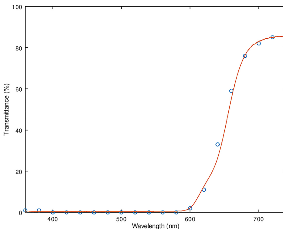
Fig. 2.4. Transmission spectrum of a Roscolux, R27, Medium Red filter (Roscolux, USA) as measured by the optical setup shown in Fig. 2.3 (—), manufacturer's data given every 20 nm is overlaid (o).
