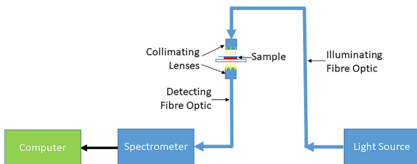
Fig. 2.1. Schematic diagram of the key components of the optical system for measuring the UV-Vis-NIR spectral absorbance of control, Plasmodium and Trypanosoma infected mouse blood after Firdous et al. 2012 [23].
