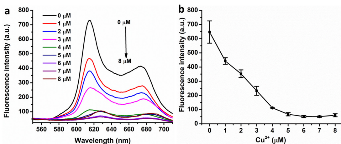
Fig. 3. (a) Fluorescence emission spectra of different Cu 2+ concentrations (0–8 \mu M). (b) The fluorescence intensity change at the maximum emission wavelength (615 nm) under different Cu 2+ concentrations.
