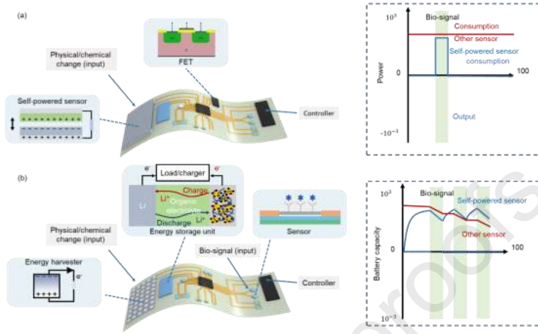
Fig. 2 Two typical modes of closed-loop system based on self-powered technology. (a) Diagram of a self-powered sensor for closed-loop control system. (b) Diagram of a closed-loop self-powered sensing and controlling system
