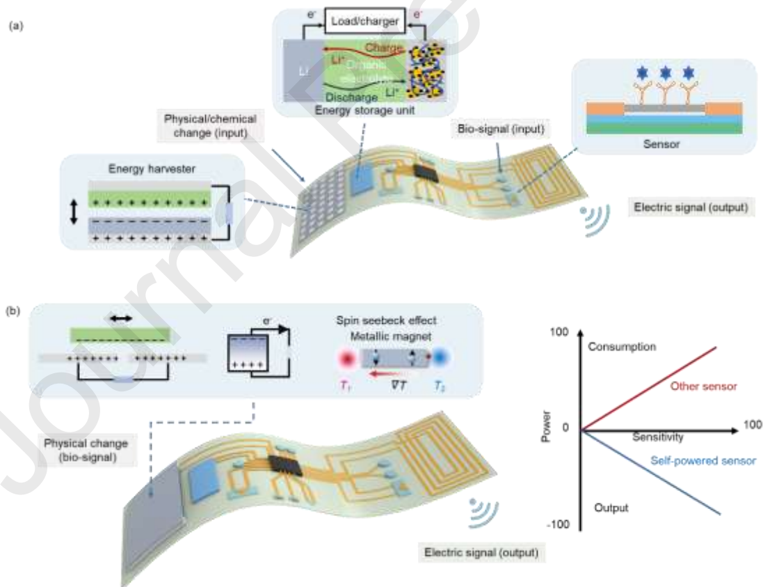
Fig. 1 Two typical modes of self-powered technology for the next generation of biosensors. (a)
