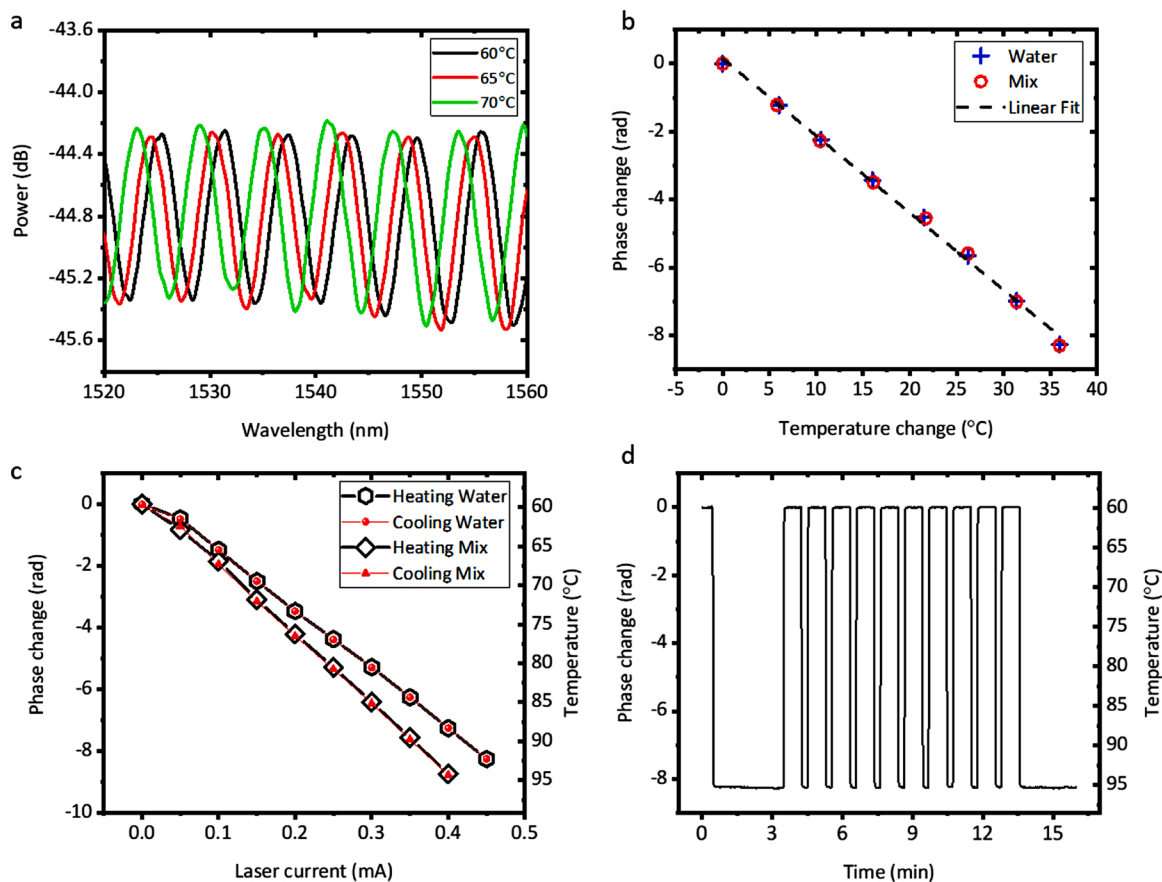
Fig. 2. (a) Fabry-Perot interference spectra of the water-filled microcavity at different ambient temperatures. (b) Phase change of the Fabry-Perot interference spectra (water and qPCR mix microcavity) at different ambient temperatures. (c) Phase change of the Fabry-Perot interference spectra with different laser current. (d) Phase change and corresponding temperature of the Fabry-Perot interference spectra (qPCR mix microcavity) with laser current cycling.
