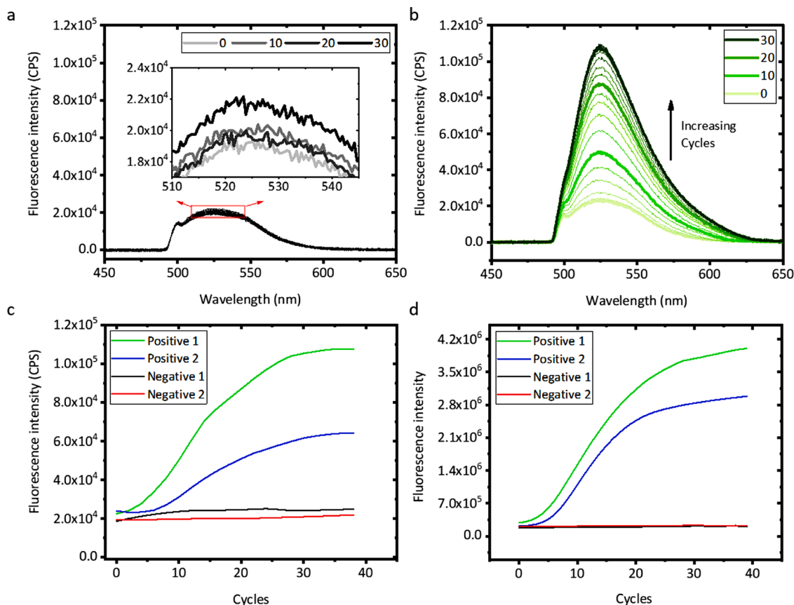
Fig. 3. Fluorescence spectra and amplification curves for increasing qPCR cycles. (a) NTC, (b) target, (c) amplification curve from the all-fiber qPCR system, and (d) amplification curve from the Viia™ 7 Real-Time PCR system. (c), (d) “1” and “2” are replicates.
