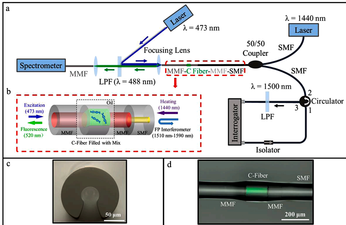
Fig. 1. Schematic diagram of the all-fiber qPCR system. (b) Schematic diagram of the C-fiber cavity. (c) Microscope cross sectional image of the C-fiber. (d) Microscope image of the C-fiber cavity filled with 6-Carboxyfluorescein (6-FAM) fluorescent solution. The green inside the C-fiber is the generated fluorescence with the excitation source turned on. Acronyms: LPF, Long Pass Filter; SMF, Single Mode Fiber; MMF, Multimode Fiber (For interpretation of the references to colour in this figure legend, the reader is referred to the web version of this article).
