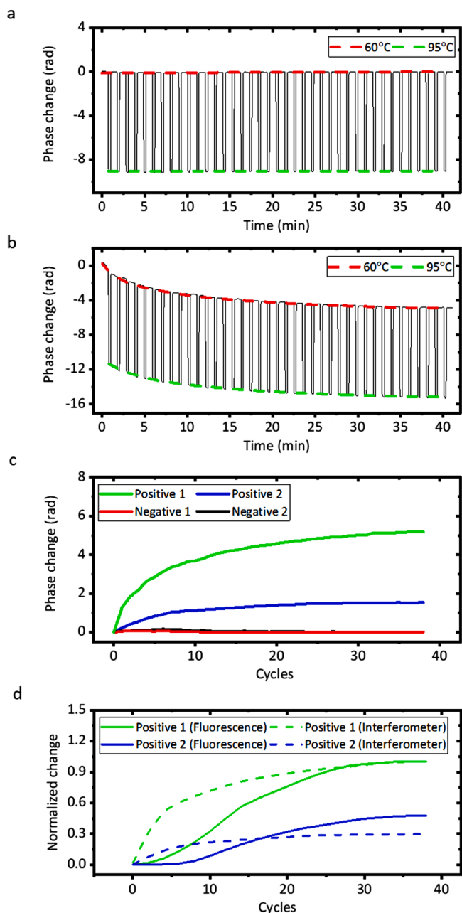
Fig. 4. (a) Phase change for increasing qPCR cycles (negative control), (b) phase change for increasing qPCR cycles (target), (c) phase-cycles amplification curve, (d) amplification curve for the fluorescence detection (solid lines) compared to the detection of the Fabry-Perot interferometer phase change (dashed lines). The curves for replicate “1” were normalized to unity for both the interferometer response and the fluorescence response (Positive 1 in Fig. 3c and Positive 1 in Fig. 4c). The values for the replicate “2” test (Positive 2 in Fig. 3c and Positive 2 in Fig. 4c) were scaled with the same normalization.
