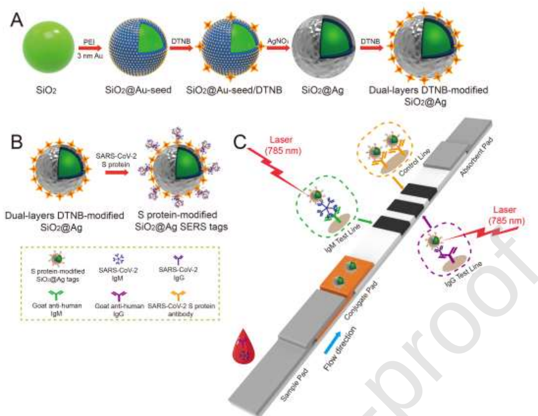
Scheme 1. (A) Schematic diagram of the preparation of the dual-layers DTNB-modified \text{SiO}_2@\text{Ag} NPs. (B) Preparation of SARS-CoV-2 S protein-modified \text{SiO}_2@\text{Ag} SERS tags. (C) Operating principle of the high-sensitivity and simultaneous analysis of anti-SARS-CoV-2 IgM/IgG via the SERS-LFIA strip.
