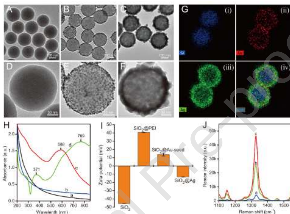
Fig. 1. HRTEM images of the prepared (A) \text{SiO}_2 NPs, (B) \text{SiO}_2@\text{Au} -seed NPs, and (C) \text{SiO}_2@\text{Ag} NPs with their corresponding enlarged images in (D), (E), and (F), respectively. (G) Element mapping results of the \text{SiO}_2@\text{Ag} NPs. UV-vis spectra (H) and zeta potentials (I) of the as-synthesized products from each stage. (J) SERS intensities of (a) \text{SiO}_2@\text{Au} -seed/DTNB NPs, (b) \text{SiO}_2@\text{Ag} /DTNB NPs, and (c) dual-layers DTNB-modified \text{SiO}_2@\text{Ag} NPs.
