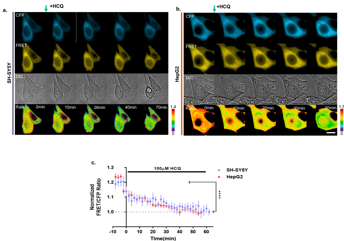
Fig. 4. ACE2 biosensor specificity in SY5Y and HepG2 cells. (a–b) Time-lapse CFP, FRET, DIC, and FRET/CFP ratio images of the ACE2 biosensor in SH-SY5Y and HepG2 cells treated with 100 \mu\text{M} HCQ, respectively. Hot and cold colors indicate high and low endogenous ACE2 and RBD affinities, respectively (scale bar = 10 \mu\text{m} ). (c) Time courses of the normalized FRET/CFP ratios of the ACE2 biosensor in SH-SY5Y (blue-violet, n = 7 ) and HepG2 (red, n = 10 ) cells treated with 100 \mu\text{M} HCQ. All error bars represent SEM (**** p < 0.0001 ).
