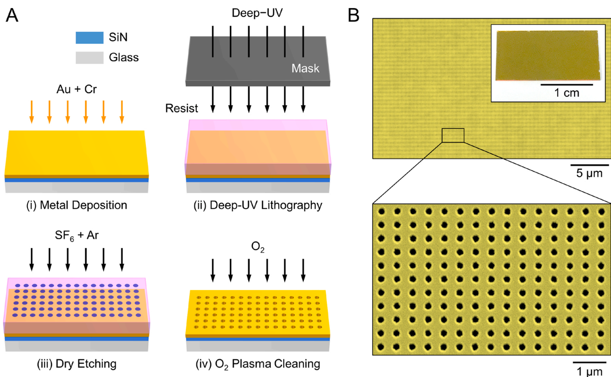
Fig. 2. (A) Schematic illustration of the wafer-scale and low-cost fabrication method based on deep-UV lithography for high-resolution plasmonic nanohole arrays. The corresponding device parameters: Hole diameter = 190 nm, Array periodicity = 450 nm, Au thickness = 120 nm, Cr thickness = 5 nm, SiN thickness: 100 nm. (B) Top: Optical microscope image of the nanohole arrays. Top-inset: Photograph of a 2 cm × 1 cm plasmonic chip. Bottom: SEM image of the nanohole arrays.
