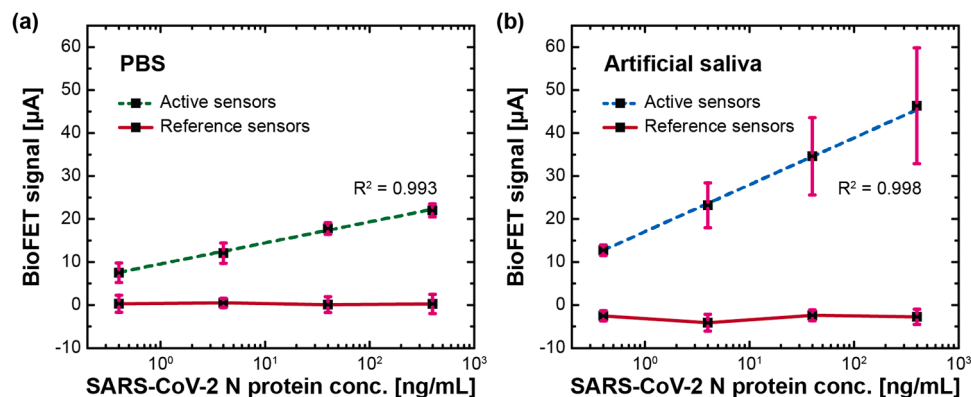
Fig. 4. COVID-19 antigen tests using EDL-gated BioFETs in (a) 1× PBS and (b) artificial saliva. Active sensors were functionalized with capture antibody, while reference sensors were unfunctionalized. SARS-CoV-2 N protein concentration varied from 0.4, 4, 40, to 400 ng/mL. Error bars represent ± 1σ of uncertainty measured by sensors ( n = 3 ).
