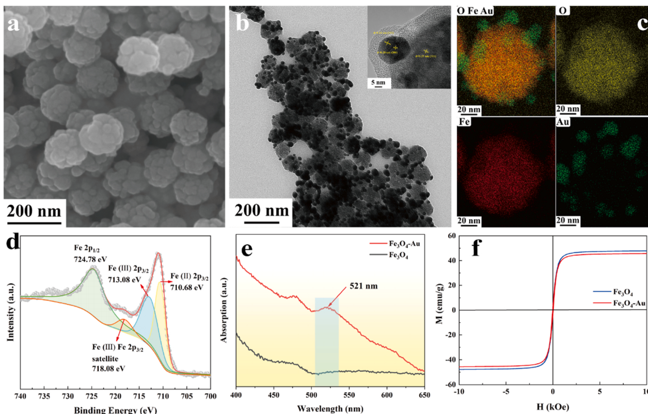
Fig. 1. Characterization of \text{Fe}_3\text{O}_4\text{-Au} nanocomposite. (a) The SEM image of \text{Fe}_3\text{O}_4 microspheres. (b) The TEM image of \text{Fe}_3\text{O}_4\text{-Au} nanocomposite. (c) The EDS mapping of \text{Fe}_3\text{O}_4\text{-Au} nanocomposite. (d) The XPS spectrum of Fe element in \text{Fe}_3\text{O}_4\text{-Au} nanocomposite. (e) The UV-Vis absorption spectra of \text{Fe}_3\text{O}_4 and \text{Fe}_3\text{O}_4\text{-Au} nanocomposite. (f) Magnetic hysteresis loops of \text{Fe}_3\text{O}_4 and \text{Fe}_3\text{O}_4\text{-Au} nanocomposite.
