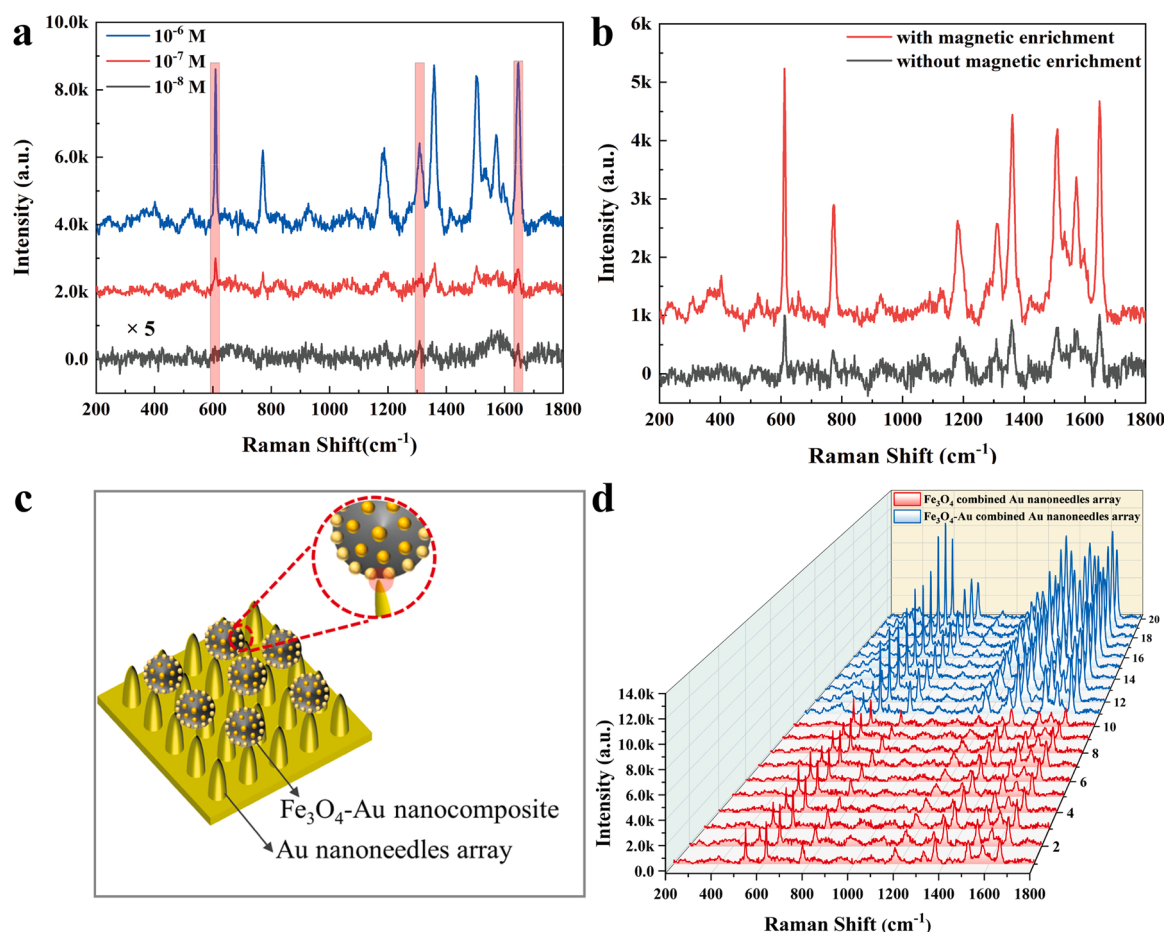
Fig. 2. The SERS performance of Fe 3 O 4 -Au nanocomposite. (a) The SERS spectra of R6G solutions with concentrations ranging from 10^{-6} M to 10^{-8} M (The “× 5” on the left side of the figure is the magnification of the Raman spectra under this scale). (b) The SERS spectra of 10^{-6} M R6G by Fe 3 O 4 -Au nanocomposite with magnetic enrichment (red line) and without magnetic enrichment (black line). (c) The schematic diagram of magnetic SERS biosensor structure which is Fe 3 O 4 -Au nanocomposite combined with Au nanoneedles array. (d) The Raman mapping image of 10^{-6} M R6G based on Fe 3 O 4 microspheres combined with Au nanoneedles array (red lines) and Fe 3 O 4 -Au nanocomposites combined with Au nanoneedles array (blue lines).
