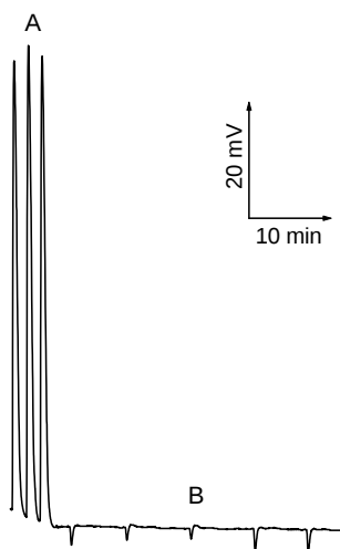
Fig. 2. Signal of the biosensor for samples of dialysate fluid injected into the FIA system without (A) and with (B) use of the cationite column. The samples contain sodium, potassium, magnesium and calcium cations at levels 140, 3.0, 1.0 and 2.0 mM, respectively.
