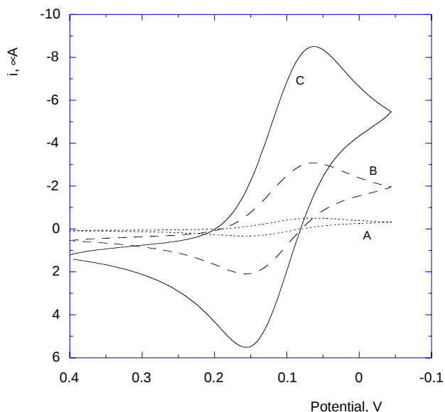
Fig. 4. Cyclic voltammograms of a 5 mM hexacyanoferrate(III) solution on a Pt electrode surface after coating the surface with SAMs: (A) 1 mM of 1-hexadecanethiol, t_{\text{SAM}} = 10 min; (b) 5 mM of 1-propanethiol, t_{\text{SAM}} = 1 h; (C) 1 mM of 1-propanethiol, t_{\text{SAM}} = 2 h.
