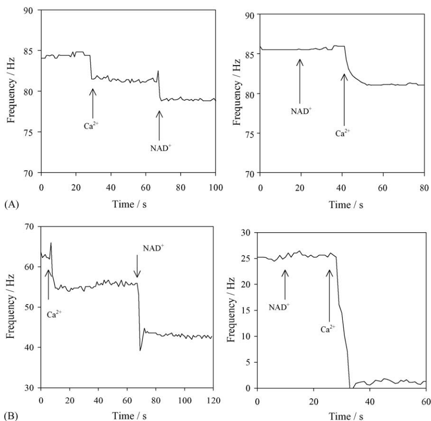
Fig. 5. Quartz crystal microbalance measurements at open circuit vs. time with a mediator modified crystal. The left column shows the successive addition of 40 mM calcium and 1 mM \text{NAD}^+ indicated by the arrows, whereas, the right column shows the opposite sequence. (A) Gold quartz crystal modified as in Fig. 1 with all nitro groups intact. (B) Modified gold quartz crystal with two activated nitro groups.
