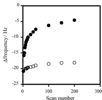
Fig. 3. Quartz crystal microbalance measurements at open circuit vs. the number of scans. Gold quartz crystal modified as in Fig. 1. Frequency changes in the absence of calcium (filled circles), in the presence of 0.1 M calcium (empty circles).
