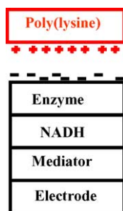
Scheme 1. Representation of the supramolecular structure (catalyst/ \text{Ca}^{2+} / \text{NAD}^+ /GDH/polylysine) at the modified glassy carbon electrode.
