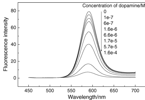
Fig. 4. Fluorescence spectra of CdSe nanocrystals in the absence and presence of different concentration of dopamine.
