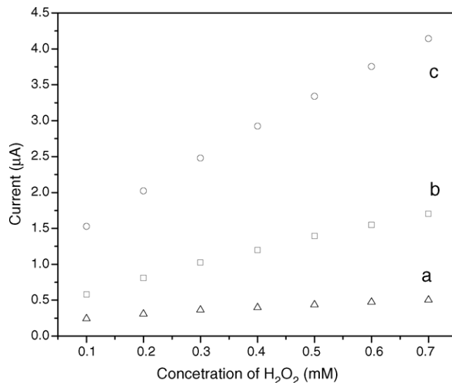
Fig. 6. Calibration curves of enzyme electrodes with different content of MWNT for concentration of \text{H}_2\text{O}_2 in the range of 0.1–0.7 mM in phosphate buffer solution (0.1 M, pH 6.9): applied potential, -0.2 V; (a) 2.5 mg \text{ml}^{-1} , (b) 5 mg \text{ml}^{-1} , and (c) 10 mg \text{ml}^{-1} .
