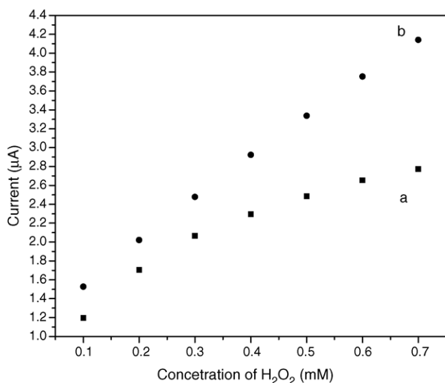
Fig. 5. Calibration curve for the concentration of \text{H}_2\text{O}_2 in the range of 0.1–0.7 mM in phosphate buffer solution (0.1 M, pH 6.9): applied potential, -0.2 V; (a) MWNTs coated GCE and (b) enzyme electrode.
