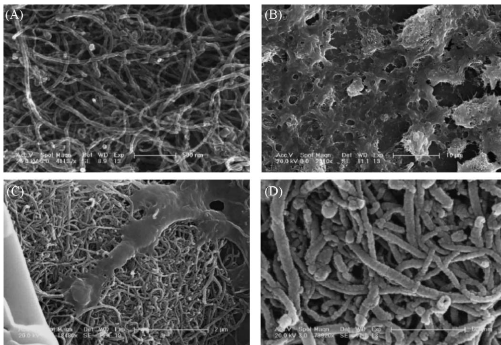
Fig. 1. FE-SEM images of MWNTs purified by 3 M HNO 3 and of MWNTs/chitosan composite films on the surface of ITO glass: (A) MWNTs purified by HNO 3 , (B) MWNTs/chitosan composite. (B), (C), and (D) corresponding to images at different locations and magnification.
