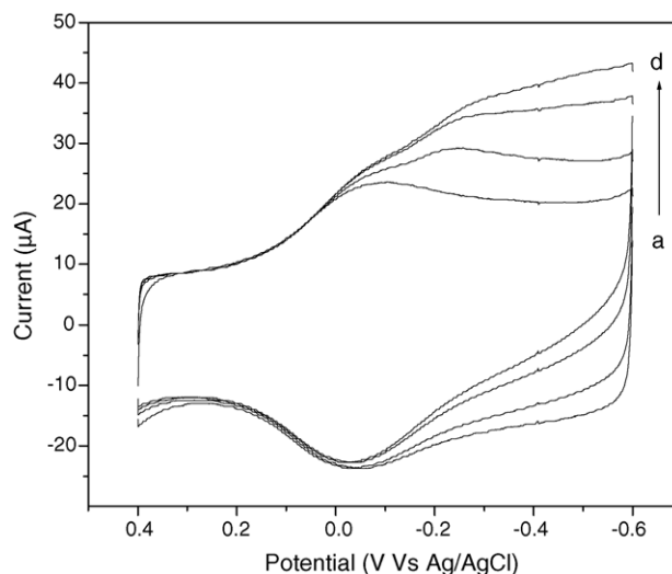
Fig. 4. Cyclic voltammograms of enzyme electrode in phosphate buffer solution (0.1 M, pH 6.9) with different amount of \text{H}_2\text{O}_2 at a scan rate of 20 \text{ mV s}^{-1} : (a) 0, (b) 0.50 \text{ mM} , (c) 1.46 \text{ mM} , and (d) 2.38 \text{ mM} .
