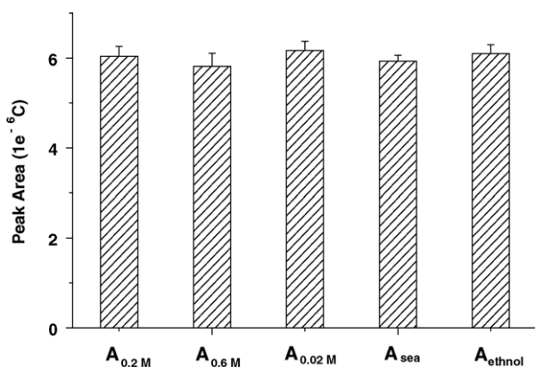
Fig. 6. Amperometric responses of the biosensors before and after the flowing pass of different solutions. The detailed experimental conditions see text. The R.S.D. of different amperometric responses is 2.31%.
