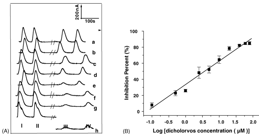
Fig. 5. Dichlorvos in simulated seawater inhibition response to the biosensor. Operating potential: 0.25 V; flow rate: 0.347 \text{ mL/min} immobilized 5 IU AChE on each electrode. Incubation time: 5 min (a) 0.1 \mu\text{M} ; (b) 1 \mu\text{M} ; (c) 5 \mu\text{M} ; (d) 10 \mu\text{M} ; (e) 20 \mu\text{M} ; (f) 40 \mu\text{M} ; (g) 60 \mu\text{M} ; (g) 80 \mu\text{M} dichlorvos. (A) The inhibition responses. (B) The working curve of inhibition responses.
