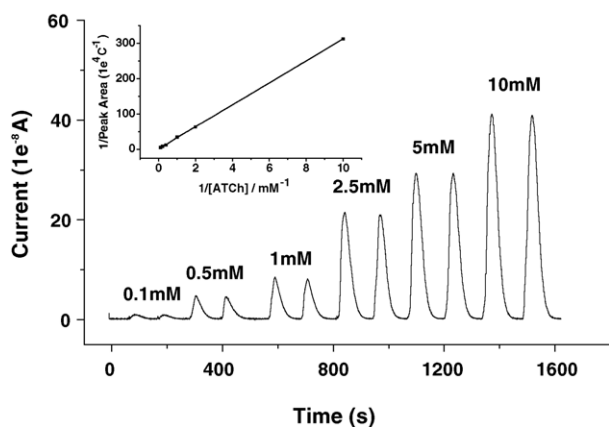
Fig. 4. Responses of the biosensor for successive injection ATCh. Inlet is the Line-weaver-Burk electrochemical representation of 1/\text{peak area} versus 1/[\text{ATCh}] . Working potential: 0.25 V vs. Ag/AgCl.
